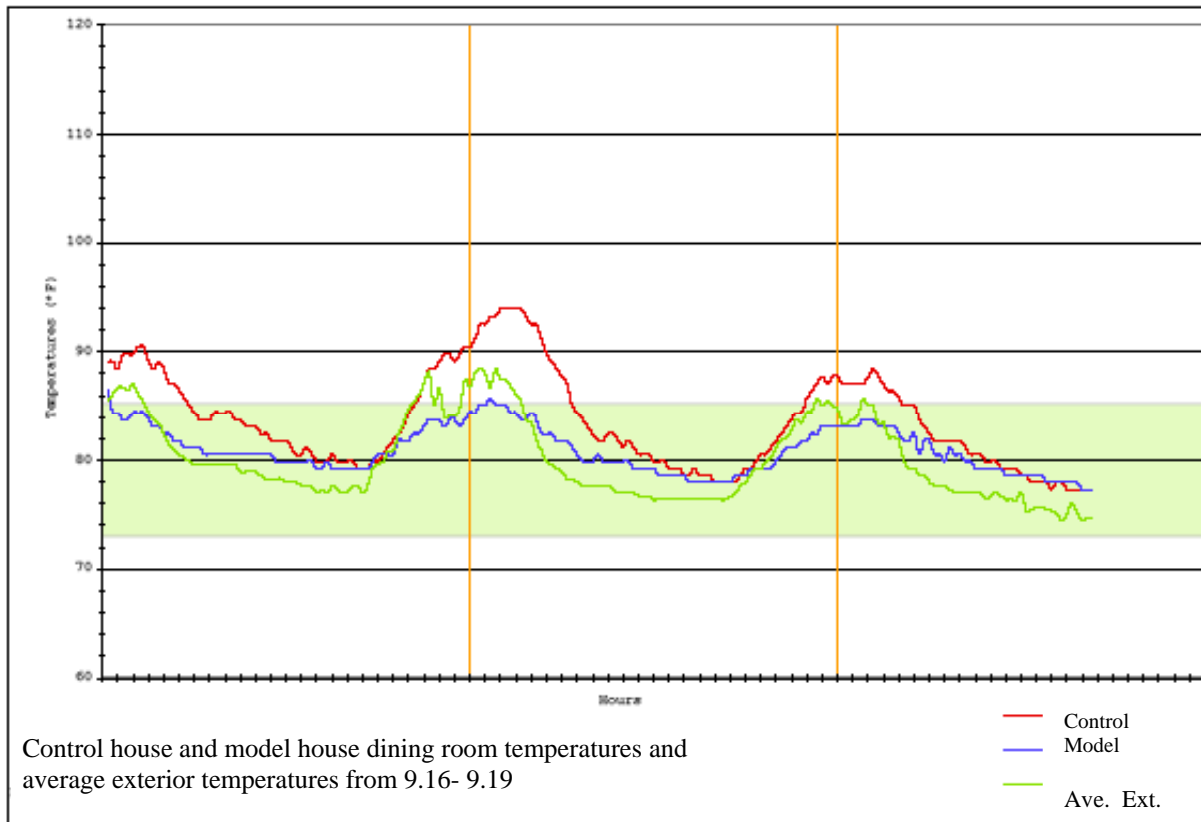
Figure 4. Temperature Monitoring Data of Exterior and Both Test Houses
