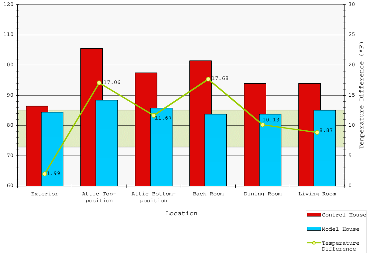
Figure 5. Comparison of Control House Temperatures versus Model House Temperatures for September 17 th at 5:15PM
