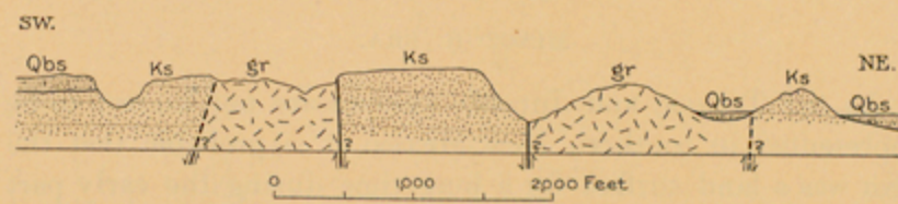
FIGURE 10.—Section across Pony Hills, showing supposed block faulting. gr, Pre-Cambrian granite; Ks, Sartén sandstone; Qbs, bolson deposits.
