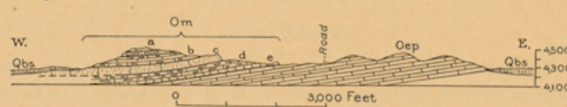
FIGURE 11.—Section across Snake Hills. Oep, El Paso limestone; Om, Montoya limestone (including a limestone with chert in large bodies; b, limestone with chert mostly in thin alternating layers; c, massive dark sandy limestone; d, cherty limestone; e, dark massive limestone with unconformity at base); Qbs, bolson deposits.
