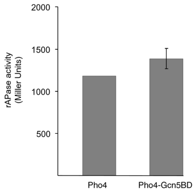
Figure 3-2. Pho4-Gcn5BD does not show increased expression in the absence of phosphate. rAPase activity assays of wild-type (Pho4) and bromodomain fusion (Pho4-Gcn5BD) strains grown in no phosphate media. The means \pm 1 standard deviation from seven independent Pho4-Gcn5BD strains are shown.
