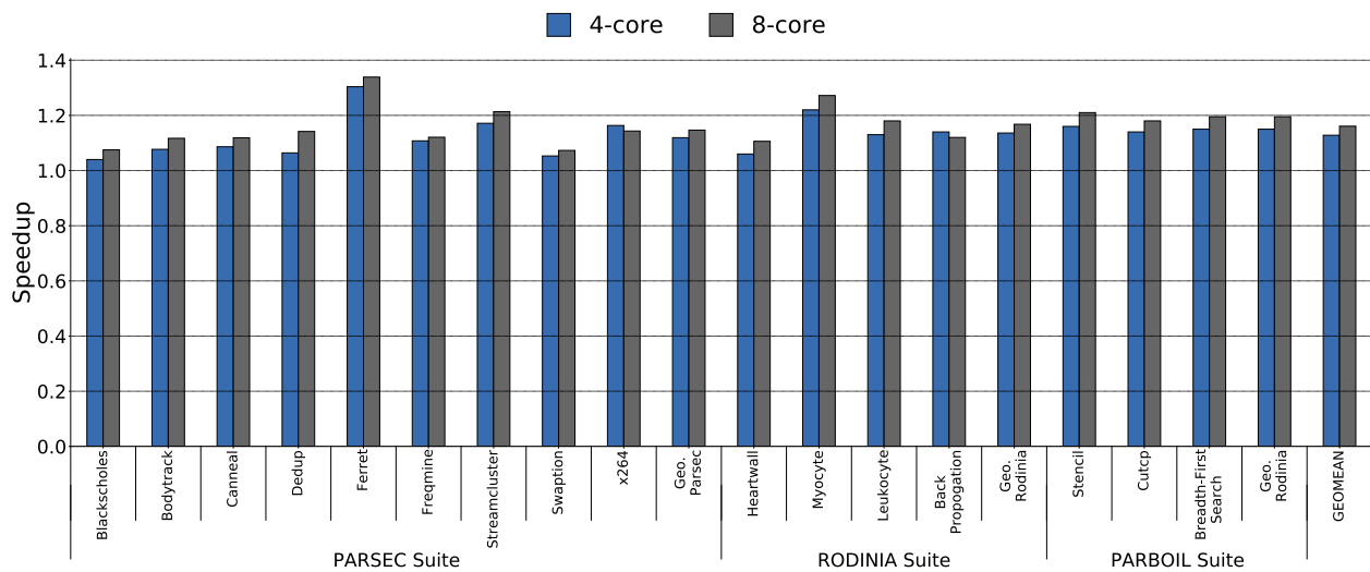
Figure 3.16: SB-Fetch speedup comparison for 4- and 8-core CMPs normalized to the baseline.
