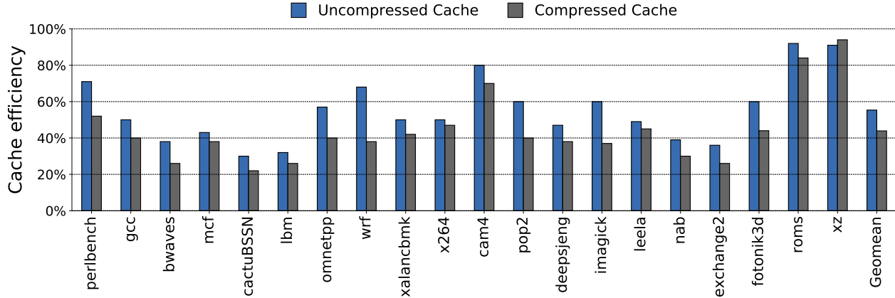
Figure 4.6: Cache efficiency.
