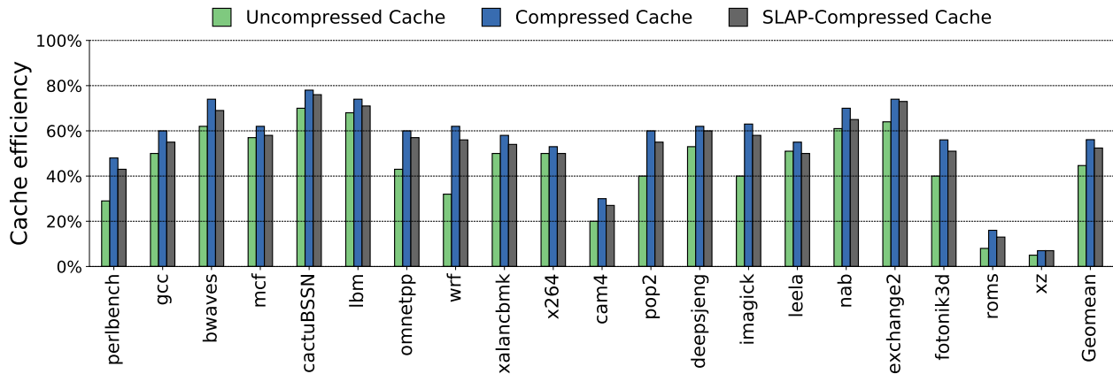
Figure 4.11: Cache efficiency.
