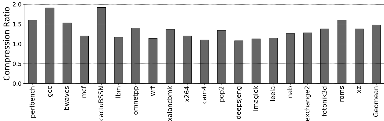
Figure 4.12: Compression Ratio.
