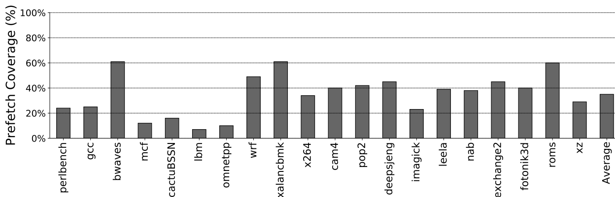
Figure 5.1: Prefetch Coverage of SPP.
