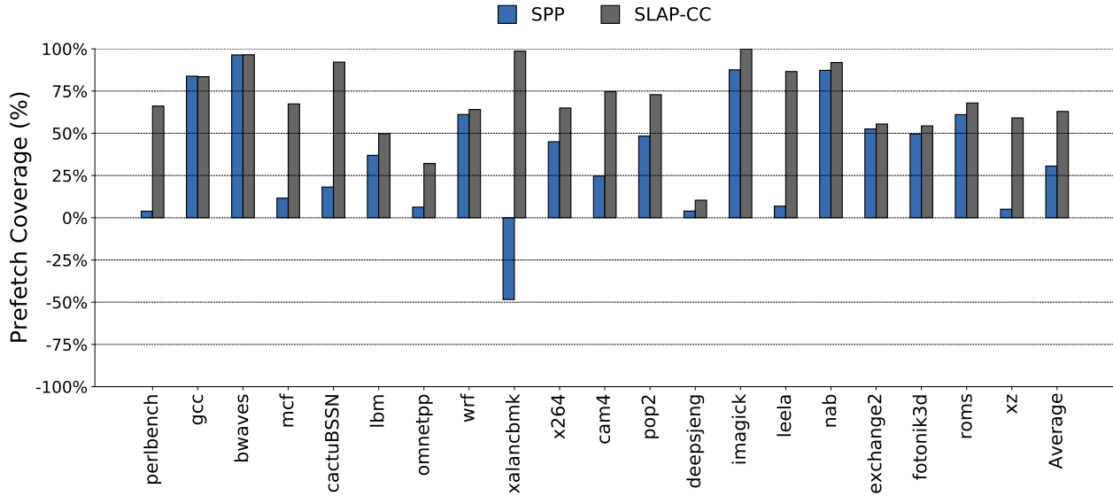
Figure 4.10: Prefetching coverage.
