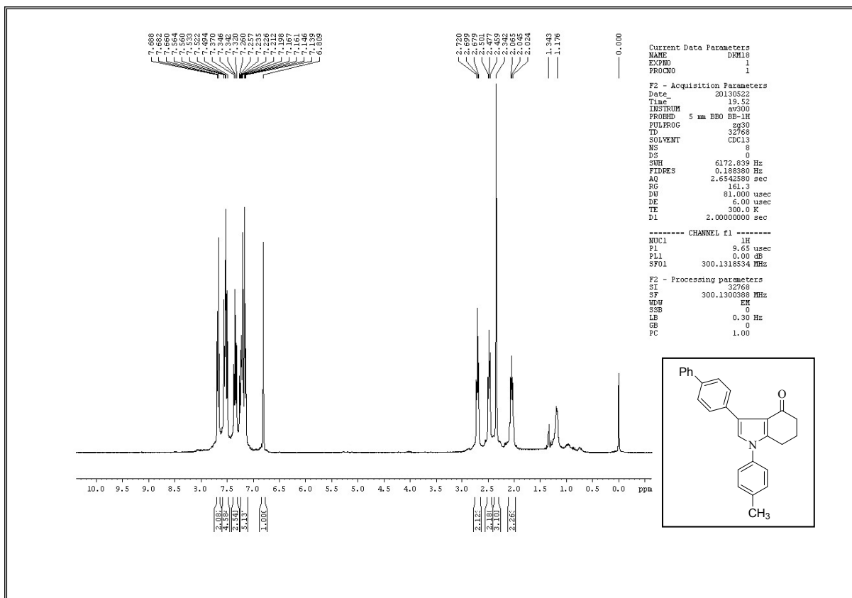
Figure 15. 1 H NMR Spectrum of 3e
