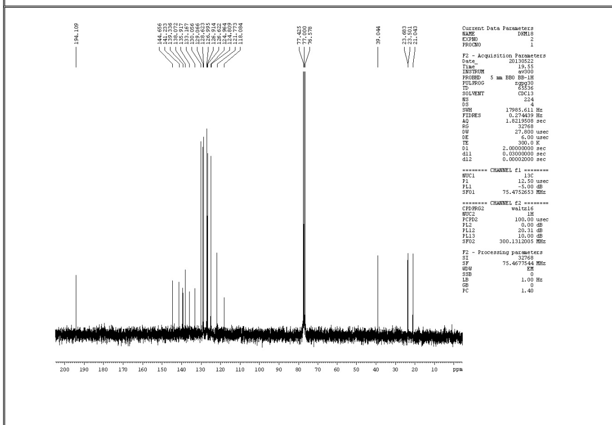
Figure 16. 13 C NMR Spectrum of 3e
