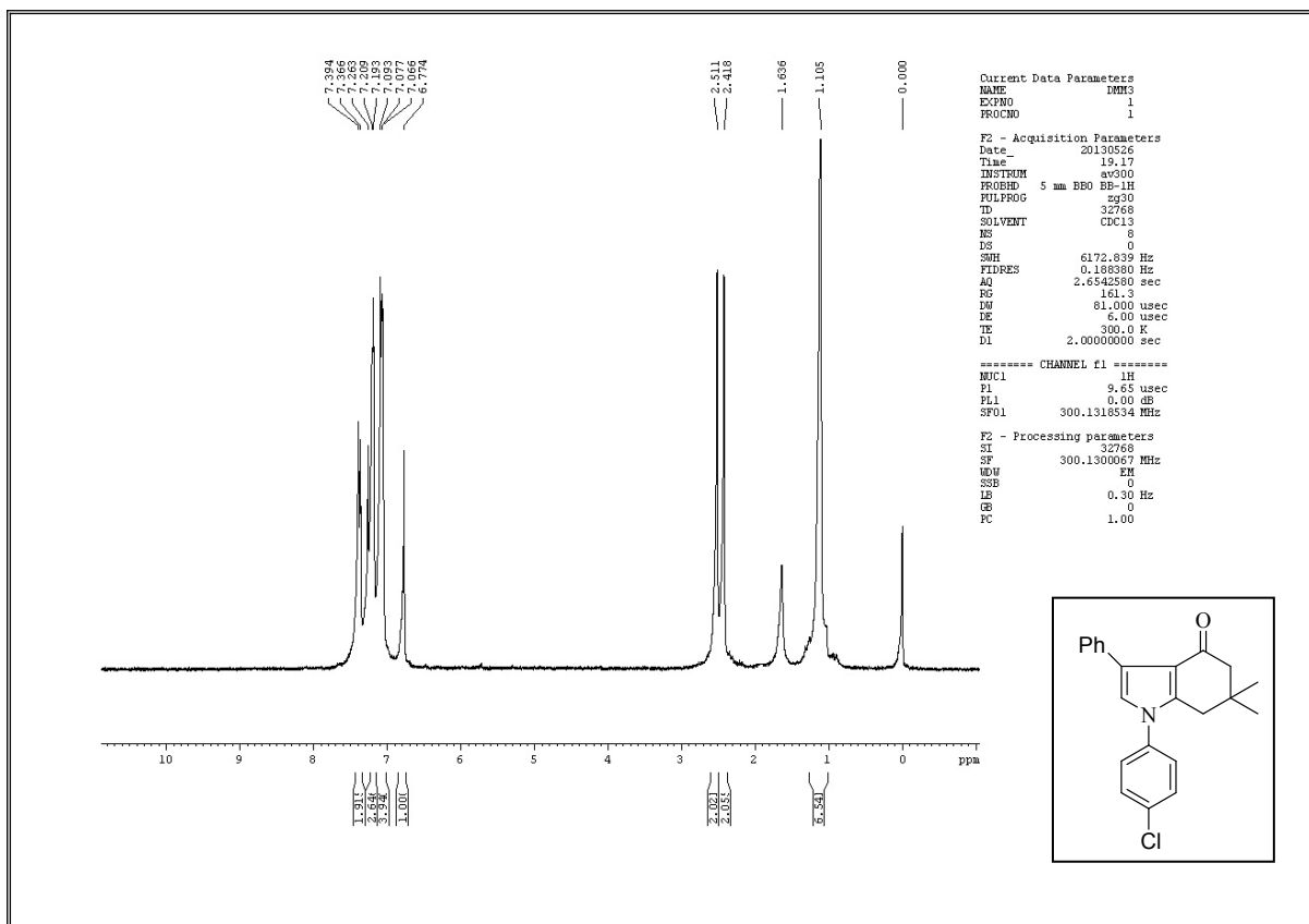
Figure 17. 1 H NMR Spectrum of 3f
