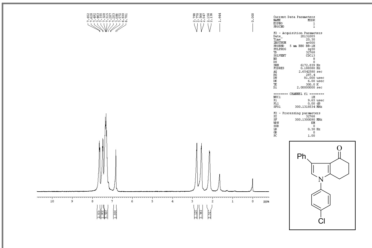
Figure 1. 1 H NMR Spectrum of 3a
