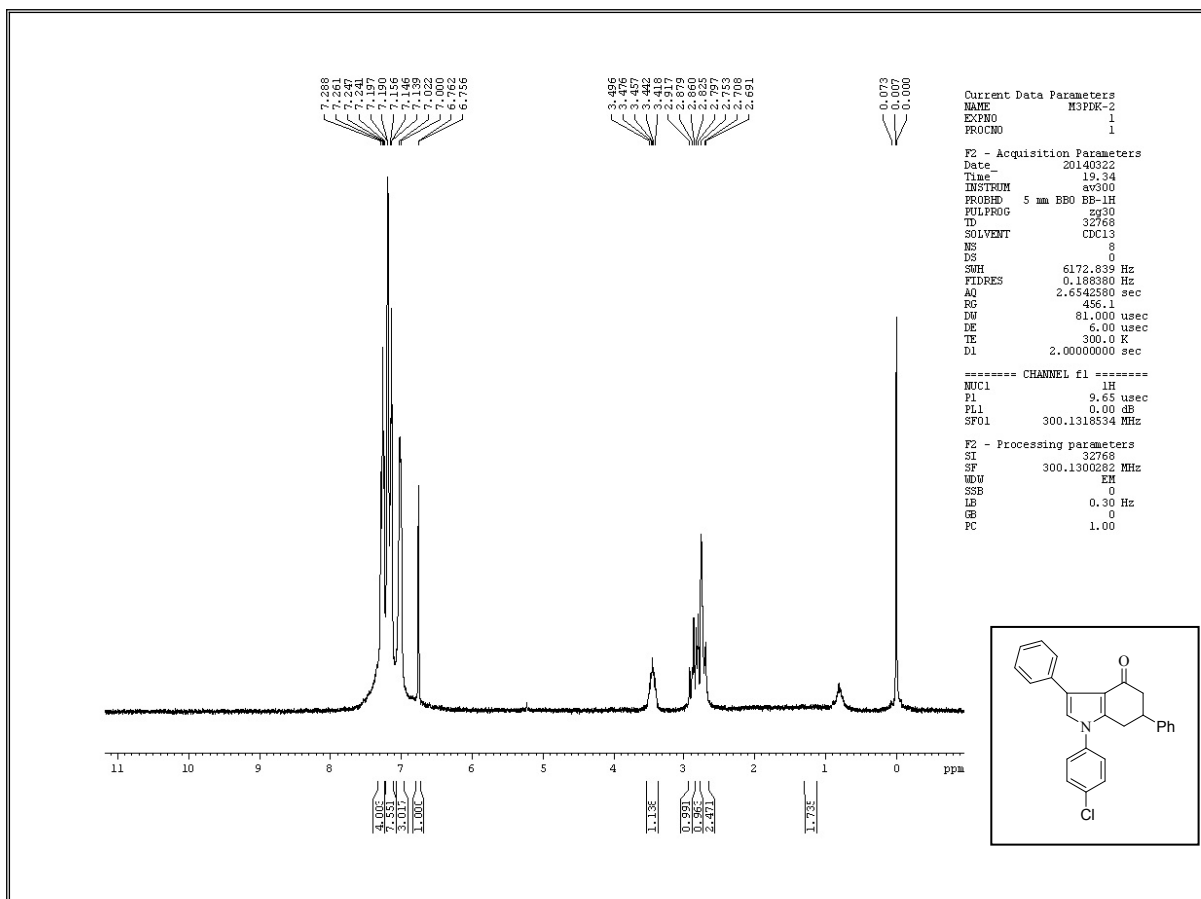
Figure 31. 1 H NMR Spectrum of 3m
