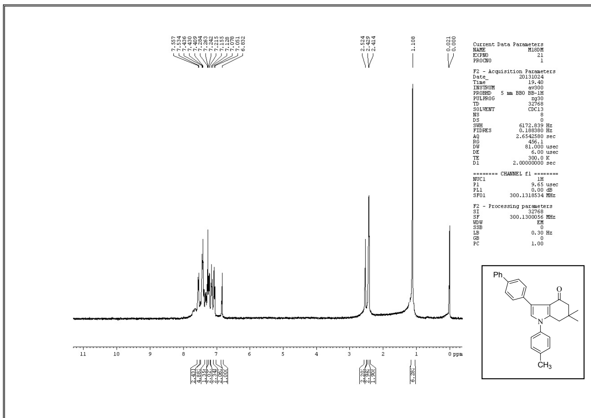
Figure 29. 1 H NMR Spectrum of 31
