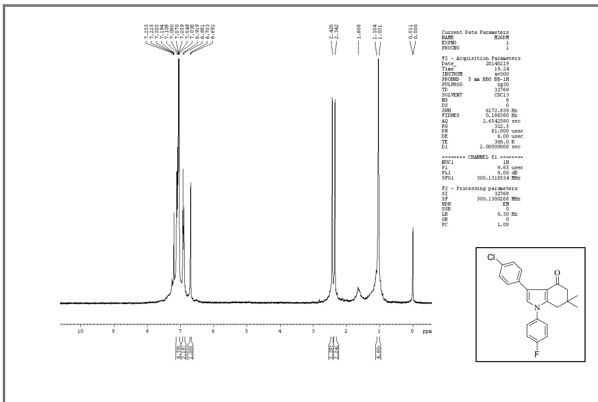
Figure 27. 1 H NMR Spectrum of 3k
