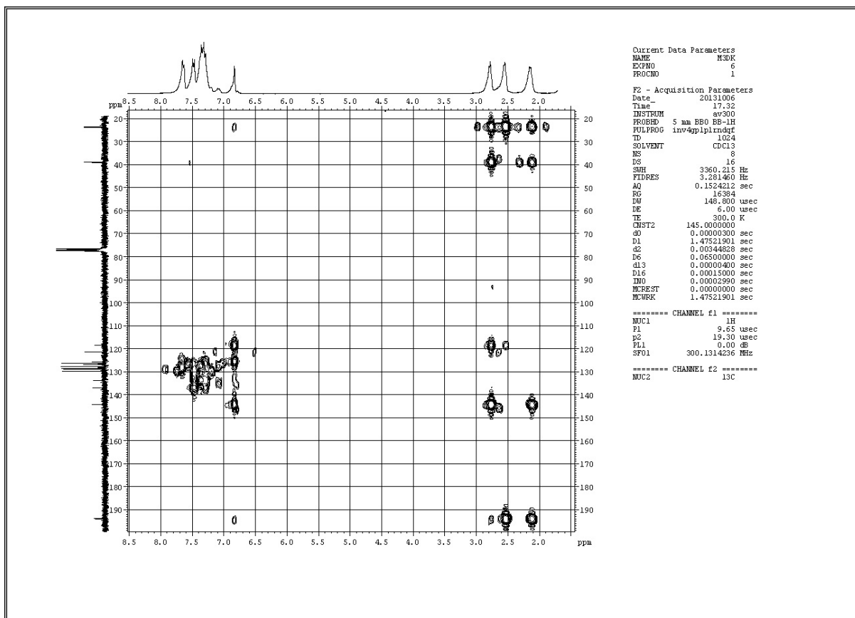
Figure 7. HMBC Spectrum of 3a
