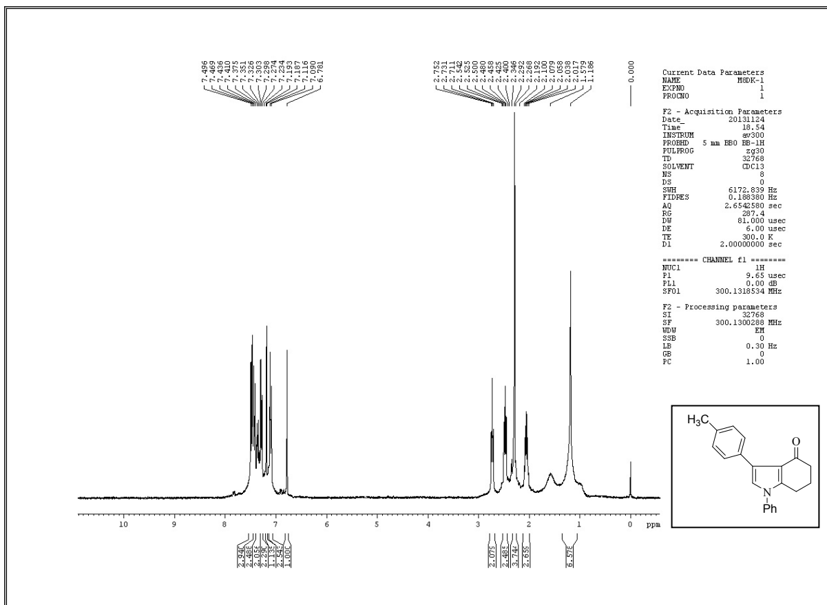
Figure 13. 1 H NMR Spectrum of 3d
