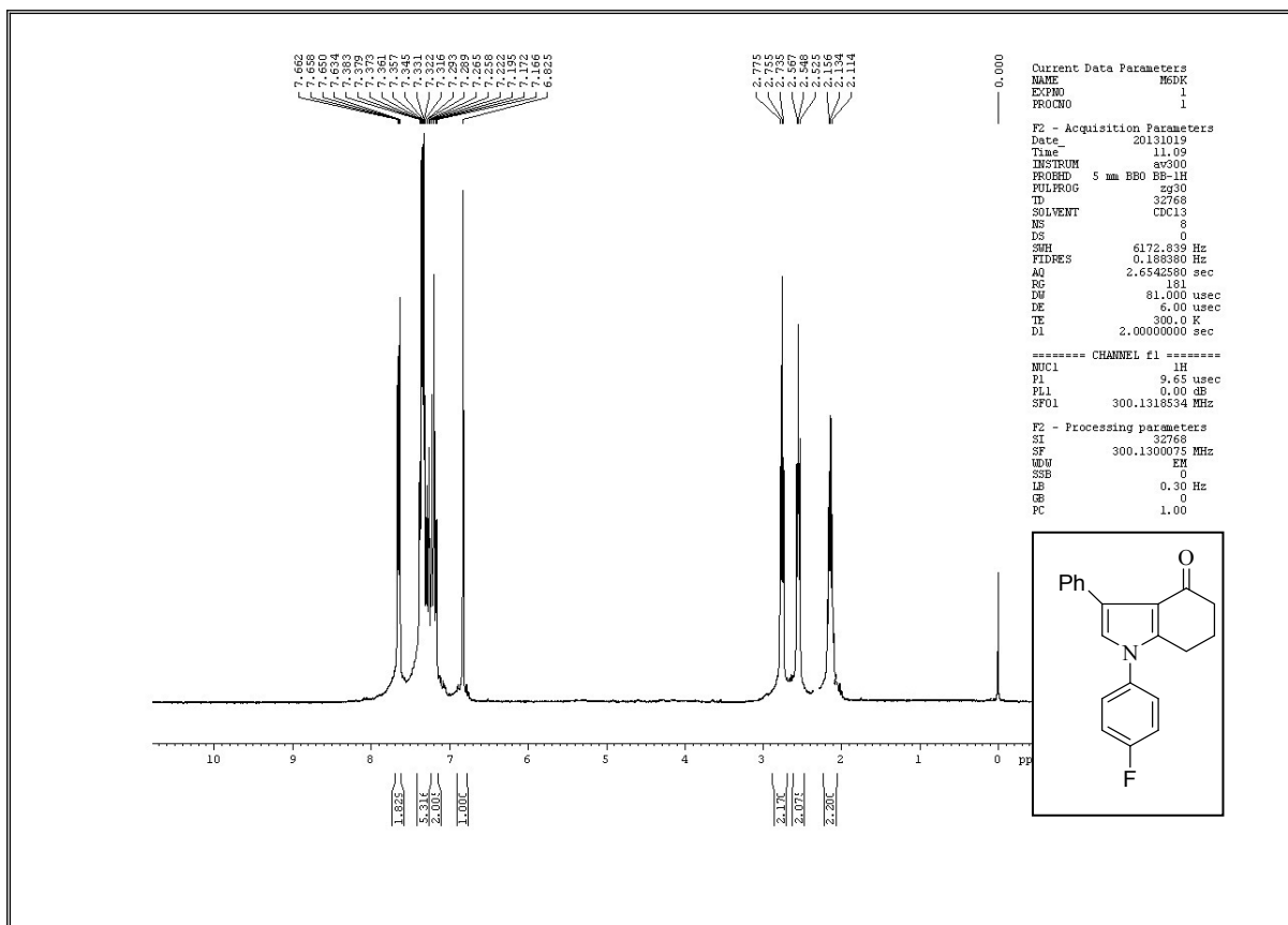
Figure 9. 1 H NMR Spectrum of 3b
