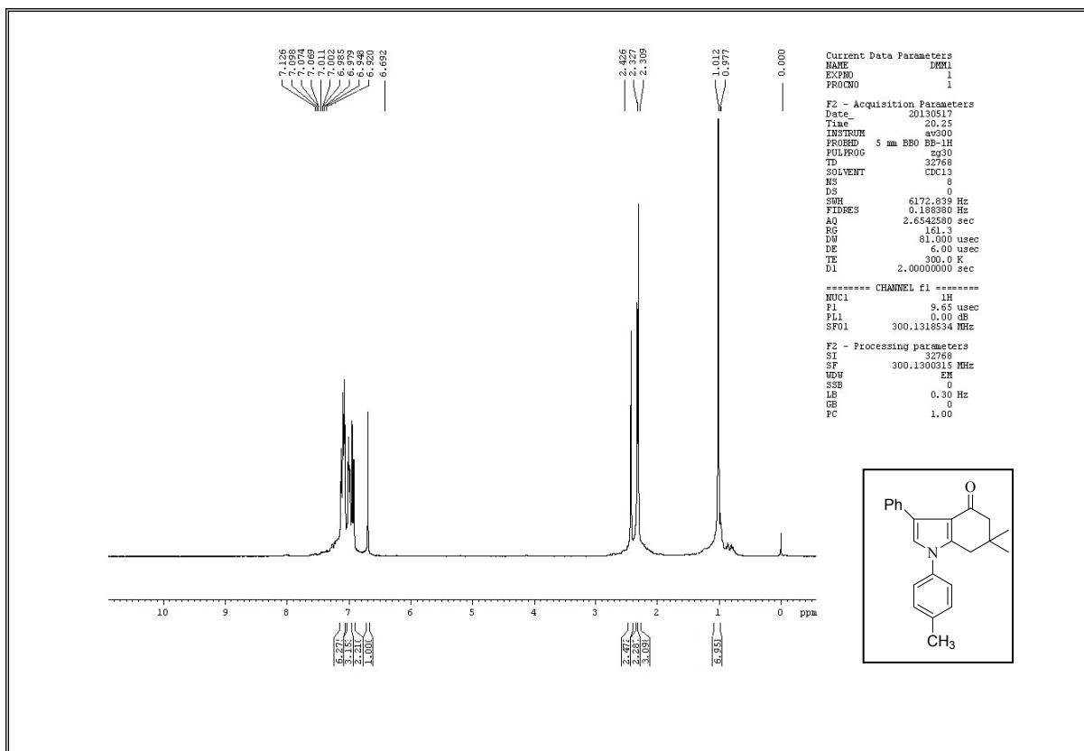
Figure 21. 1 H NMR Spectrum of 3h
