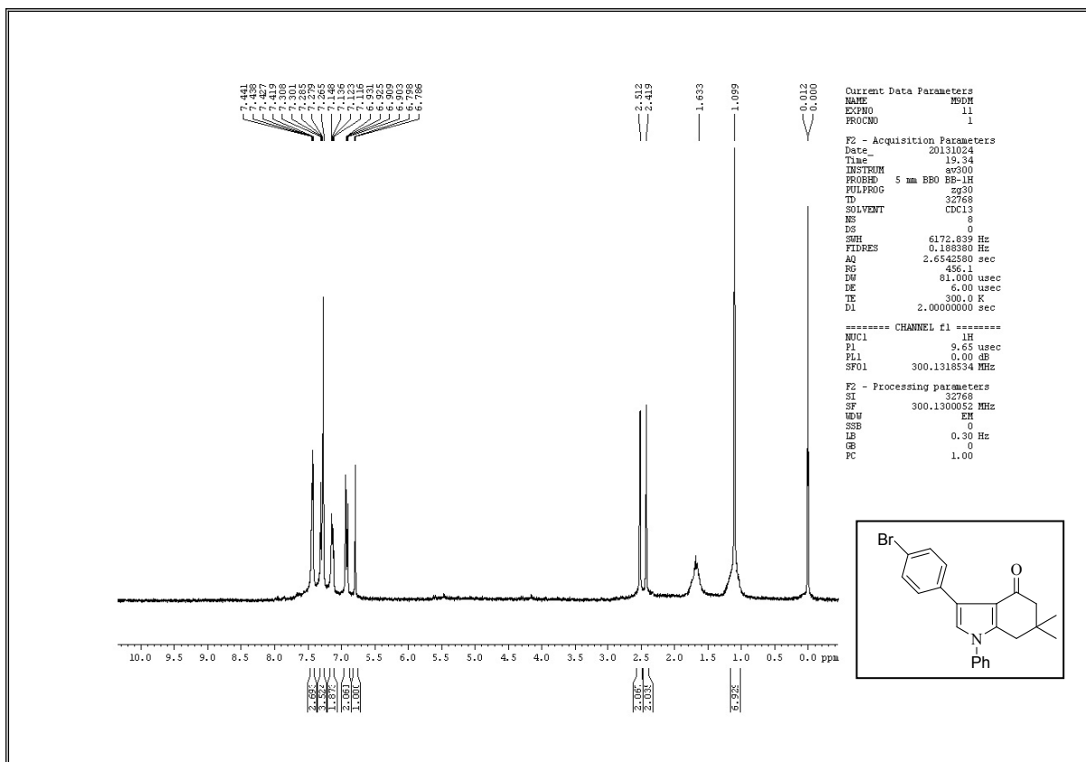
Figure 25 1 H NMR Spectrum of 3j
