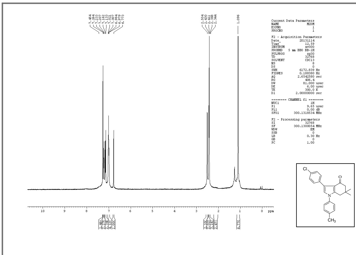
Figure 23. 1 H NMR Spectrum of 3i
