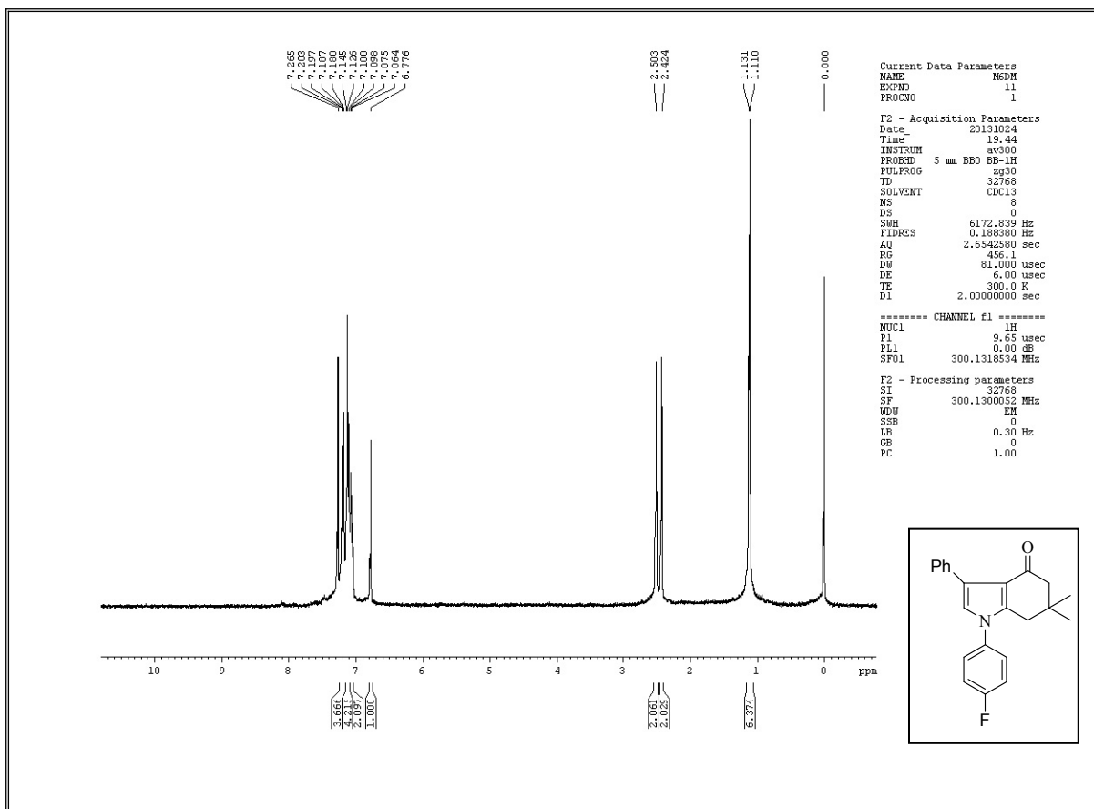
Figure 19. 1 H NMR Spectrum of 3g
