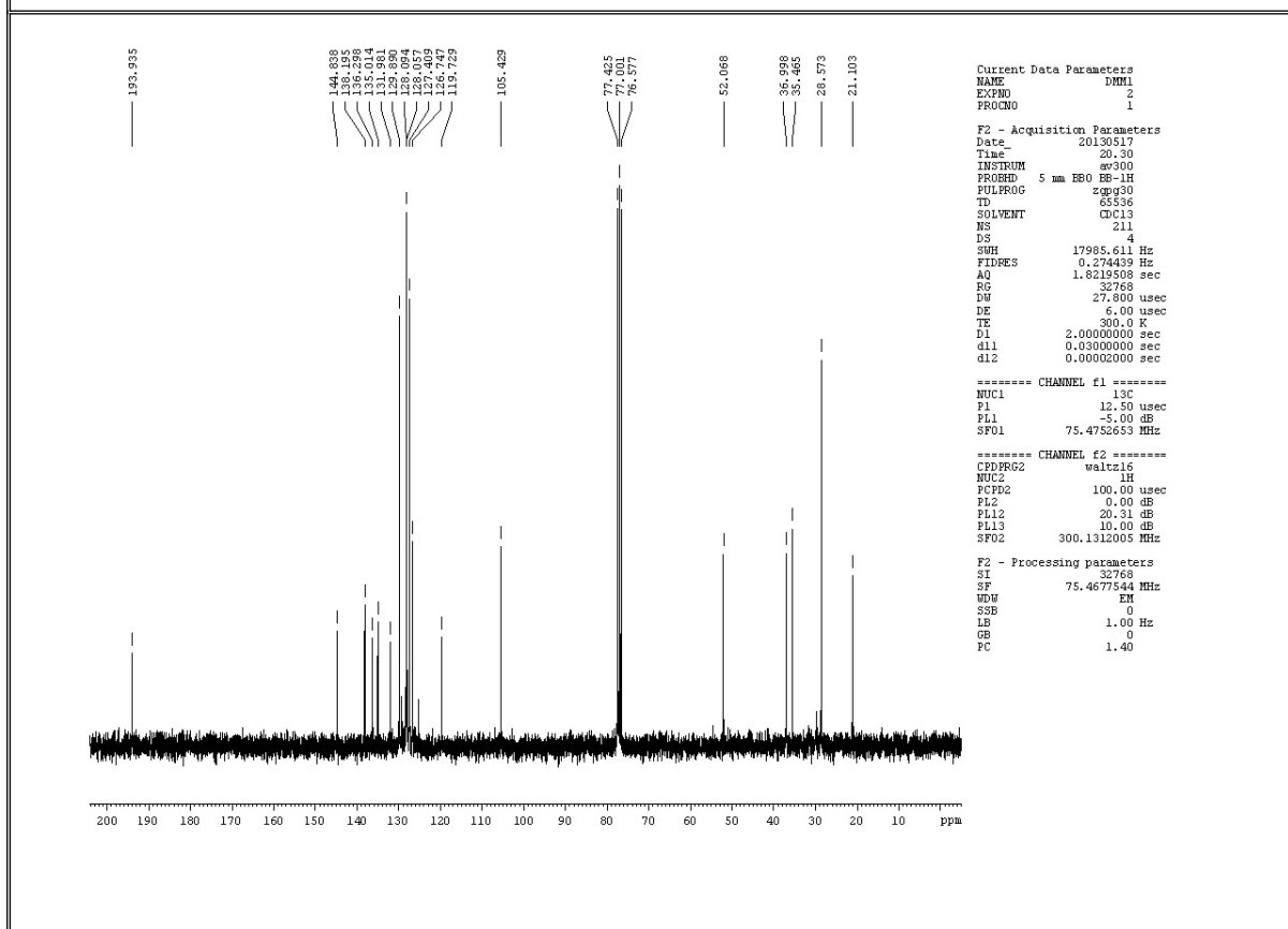
Figure 22. 13 C NMR Spectrum of 3h
