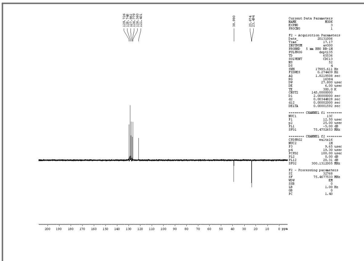
Figure 3. DEPT NMR Spectrum of 3a
