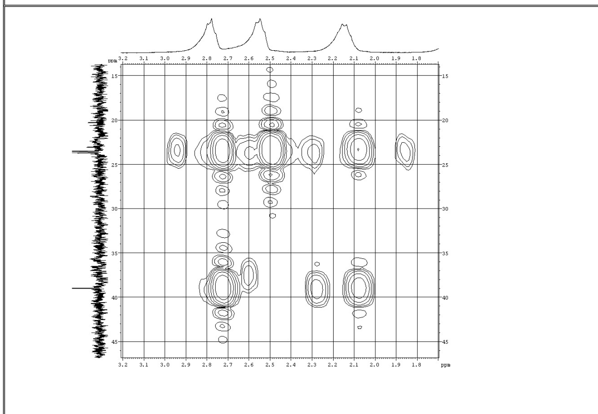
Figure 8. HMBC Spectrum of 3a (Expanded)
