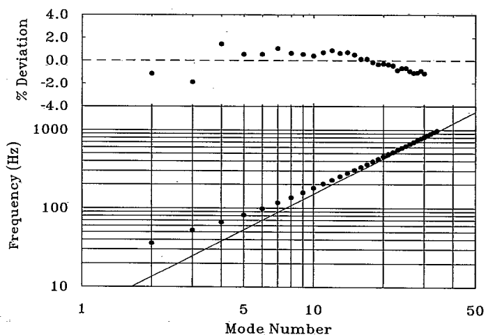
FIG. 2. The measured normal-mode frequencies plotted against mode number. The line indicates the 3/2 -power-law dependence expected for capillary waves. Also shown are the deviations determined from the fit of the experimental resonant frequencies using the normal-mode calculations.
