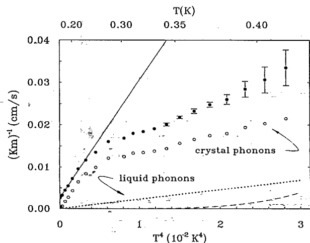
FIG. 4. (Km)^{-1} ( \bullet ) plotted vs T^4 to emphasize the phonon contribution. The solid line indicates the fit by the low-temperature phonon contribution [ 2.79T^4 \text{ cm s}^{-1} \text{ K}^{-4} ] and the T = 0 offset [ 0.0026 \text{ cm s}^{-1} ]. The crystal phonon contribution of the liquid phonons (dotted line) and rotons (dashed line) and the T = 0 offset. Error bars are derived from fits of the resonance curves of the mode with a Lorentzian line shape.
