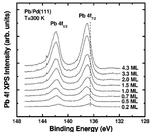
FIG. 7. Effect of Pb coverage on the Pb 4 f XPS spectra of Pb/Pd(111).
