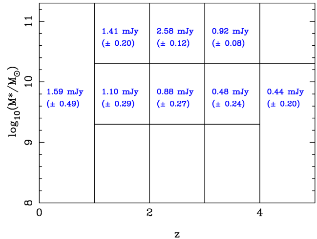
Figure 10. The distribution of 1.3-mm flux density found within the HUDF across the galaxy redshift–stellar mass plane. The figures given here combine the flux densities of the detected sources and the results of stacking in the appropriate redshift–mass bins (excluding detected sources to avoid double counting). Results are only given for bins within which stacking yielded better than a 2\sigma detection, typically corresponding to an average flux density S_{1.3} \geq 0.010 \text{mJy} . At z > 4 the HUDF contains no galaxies more massive than \log_{10}(M_*/M_\odot) = 10.3 , and so the right-hand cell in the top row is genuinely blank. The cells below \log_{10}(M_*/M_\odot) = 9.3 at 1 < z < 3 may contain additional 1.3-mm flux density, but not at a level that could be securely detected via stacking in the current image. At z < 1 and z > 4 , low sample size precludes bin subdivision by mass, and so we simply give the total flux detected via stacking of all sources in the z < 1 and z > 4 redshift bins. Addition of all the numbers in this figure, combined with an estimated contribution of \simeq 1 \text{mJy} per HUDF from sources brighter than S_{1.3} \simeq 1 \text{mJy} (equivalent to 0.8 \text{Jy deg}^{-2} ) gives an estimate of 10.6 \pm 1.0 \text{mJy} for the 1.3-mm flux density in the HUDF down to S_{1.3} \simeq 0.01 \text{mJy} (equivalent to 8.5 \pm 0.9 \text{Jy deg}^{-2} ; see Fig. 10). Of this total estimated background, \simeq 70 per cent is provided by sources with \log_{10}(M_*/M_\odot) > 9.3 in the redshift range 1 < z < 3 . Within our background estimate, \simeq 45 per cent of the flux density is contributed by the 16 individually detected sources in our ALMA image of the HUDF, with only \simeq 35 per cent added by our attempts to extend flux retrieval down to \simeq 0.01 \text{mJy} sources through stacking.
