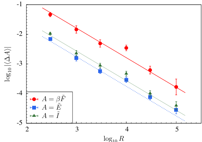
FIG. 8: (Color online) Log-log plot showing the deviations from equilibrium (systematic errors) in the dimensionless free energy, \langle\Delta\beta\tilde{F}\rangle (red circles), energy, \langle\Delta\tilde{E}\rangle (blue squares) and overlap near the origin \langle\Delta\tilde{I}\rangle (green triangles) as a function of population size R for instance J4 at T = 0.2 . The straight lines are theoretical curves based on Eqs. (22) and (23).
