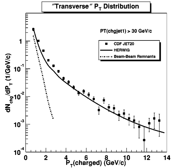
FIG. 40. Data from Fig. 37 on the transverse momentum distribution of charged particles ( p_T > 0.5 GeV/c, |\eta| < 1 ) in the “transverse” region defined in Fig. 14 for P_{T1} > 30 GeV/c compared to the QCD hard scattering Monte Carlo model predictions from HERWIG. The dashed curve shows the contribution arising from the breakup of the beam particles (“beam-beam remnants”) predicted by HERWIG.
