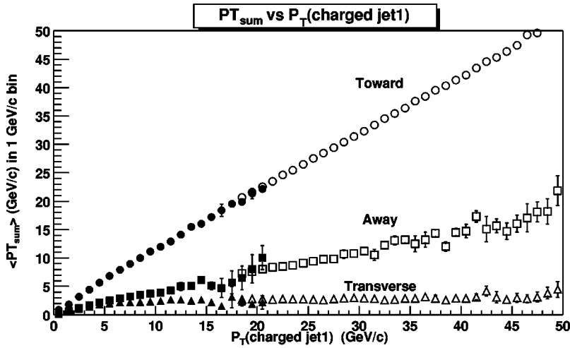
FIG. 22. The average scalar p_T sum of “toward” ( |\Delta\phi| < 60^\circ ), “transverse” ( 60^\circ < |\Delta\phi| < 120^\circ ), and “away” ( |\Delta\phi| > 120^\circ ) charged particles ( p_T > 0.5 GeV/c, |\eta| < 1 , including chgjet1) as a function of the transverse momentum of the leading charged jet. Each point corresponds to the \langle P_T \text{ sum} \rangle in a 1 GeV/c bin. The solid (open) points are the min-bias (JET20) data. The errors on the (uncorrected) data include both statistical and correlated systematic uncertainties. The “toward,” “transverse,” and “away” regions are illustrated in Fig. 14 and labeled in Fig. 16.
