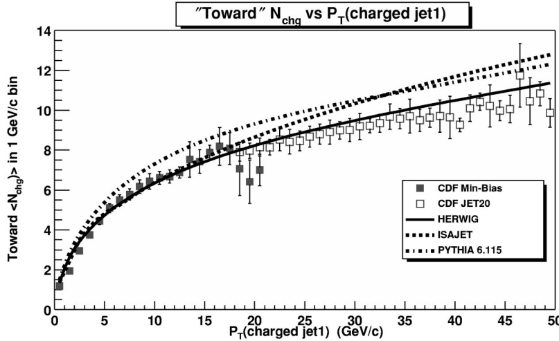
FIG. 23. Data from Fig. 21 on the average number of charged particles ( p_T > 0.5 GeV/c, |\eta| < 1 ) as a function of P_{T1} (leading charged jet) for the “toward” region defined in Fig. 14 compared with the QCD Monte Carlo model predictions of HERWIG, ISAJET, and PYTHIA 6.115.
