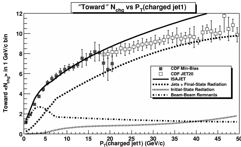
FIG. 24. Data from Fig. 21 on the average number of charged particles ( p_T > 0.5 GeV/c, |\eta| < 1 ) as a function of P_{T1} (leading charged jet) for the “toward” region defined in Fig. 14 compared with the QCD Monte Carlo model predictions of ISAJET. The predictions of ISAJET are divided into three categories: charged particles that arise from the breakup of the beam particles (“beam-beam remnants”), charged particles that arise from initial-state radiation, and charged particles that result from the outgoing jets plus final-state radiation (see Fig. 1).
