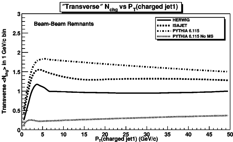
FIG. 36. QCD Monte Carlo model predictions from HERWIG, ISAJET, PYTHIA 6.115, and PYTHIA 6.115 with no multiple parton scattering (no MS) for the average number of charged particles ( p_T > 0.5 GeV/c, |\eta| < 1 ) as a function of P_{T1} (leading charged jet) for the “transverse” region defined in Fig. 14 arising from the breakup of the beam particles (“beam-beam remnants”). For PYTHIA the “beam-beam remnants” include contributions from multiple parton scattering (see Fig. 2).
