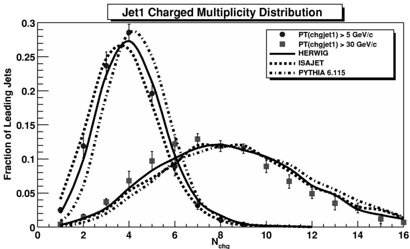
FIG. 5. Multiplicity distribution of charged particles ( p_T > 0.5 GeV/c, |\eta| < 1 ) within chgjet1 (leading charged jet) for P_{T1} > 5 and 30 GeV/c compared with the QCD Monte Carlo model predictions of HERWIG, ISAJET, and PYTHIA 6.115. This plot shows the percentage of events in which the leading charged jet ( R=0.7 ) contains N_{\text{chg}} charged particles. The P_{T1} > 5 GeV/c points are min-bias data and the P_{T1} > 30 GeV/c points are JET20 data.
