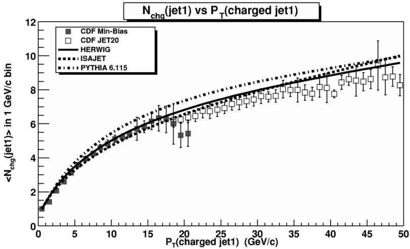
FIG. 4. The average number of charged particles ( p_T > 0.5 GeV/c, |\eta| < 1 ) within the leading charged jet ( R=0.7 ) as a function of the transverse momentum of the leading charged jet compared with the QCD Monte Carlo models predictions of HERWIG, ISAJET, and PYTHIA 6.115. The solid (open) points are min-bias (JET20) data.
