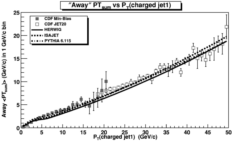
FIG. 26. Data from Fig. 22 on the average scalar p_T sum of charged particles ( p_T > 0.5 GeV/c, |\eta| < 1 ) as a function of P_{T1} (leading charged jet) for the “away” region defined in Fig. 14 compared with the QCD Monte Carlo model predictions of HERWIG, ISAJET, and PYTHIA 6.115.
