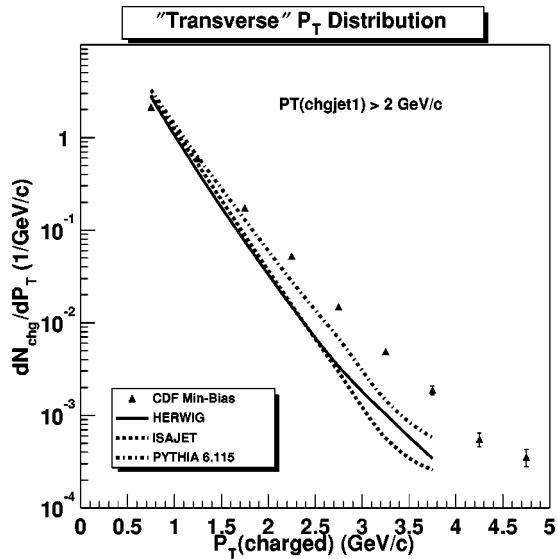
FIG. 39. Data from Fig. 37 on the transverse momentum distribution of charged particles ( p_T > 0.5 GeV/c, |\eta| < 1 ) in the “transverse” region defined in Fig. 14 for P_{T1} > 2 GeV/c compared to the QCD hard scattering Monte Carlo model predictions from predictions from HERWIG, ISAJET, and PYTHIA 6.115.
