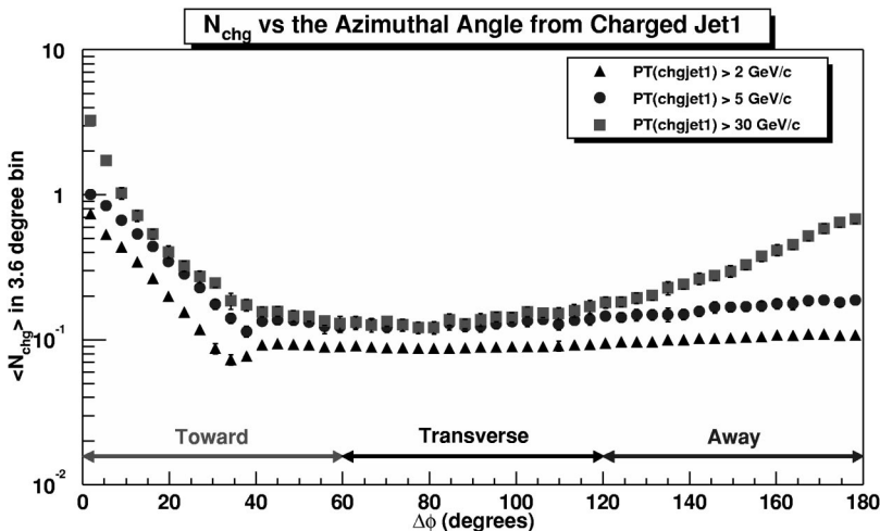
FIG. 15. Average number of charged particles ( p_T > 0.5 \text{ GeV}/c , |\eta| < 1 ) as a function of the relative azimuthal angle, \Delta\phi , between the particle and \text{chgjet1} (leading charged jet) for P_{T1} > 2 \text{ GeV}/c , 5 \text{ GeV}/c , and 30 \text{ GeV}/c . Each point corresponds to the \langle N_{\text{chg}} \rangle in a 3.6^\circ bin. The P_{T1} > 2 \text{ GeV}/c and 5 \text{ GeV}/c points are the min-bias data and the P_{T1} > 30 \text{ GeV}/c points are JET20 data. The “toward,” “transverse,” and “away” regions defined in Fig. 14 are labeled.
