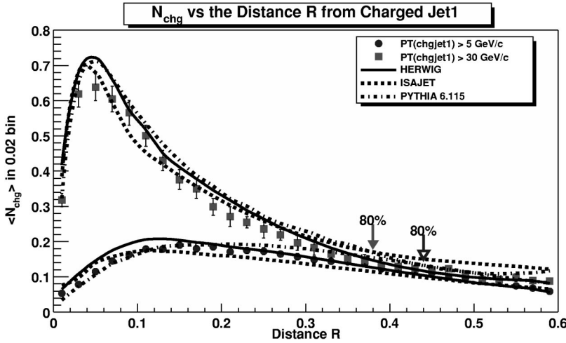
FIG. 8. Charged multiplicity distribution in the radial distance R in \eta - \phi space from chgjet1 (leading charged jet) for charged particles with p_T > 0.5 GeV/c and |\eta| < 1 when P_{T1} > 5 and 30 GeV/c. The points are \langle N_{\text{chg}} \rangle in a \Delta R = 0.02 bin (see Fig. 7). The P_{T1} > 5 GeV/c points are min-bias data and the P_{T1} > 30 GeV/c points are JET20 data. The data are compared with the QCD Monte Carlo model predictions of HERWIG, ISAJET, and PYTHIA 6.115. For an average charged jet with P_{T1} > 5 GeV/c ( > 30 GeV/c), 80% of the charged particles lie within R = 0.44 (0.38) as marked by the arrows.
