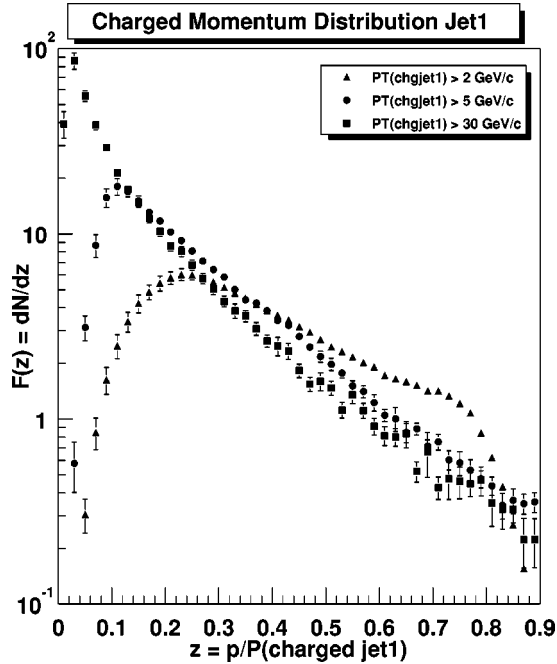
FIG. 10. Momentum distribution of charged particles ( p_T > 0.5 GeV/c, |\eta| < 1 ) within chgjet1 (leading charged jet). The points are the charged number density, F(z) = dN_{\text{chg}}/dz , where z = p/P(\text{chgjet1}) is the ratio of the charged particle momentum to the charged momentum of chgjet1. The integral of F(z) is the average number of particles within chgjet1 (see Fig. 5). The P_{T1} > 2 GeV/c and 5 GeV/c points are min-bias data and the P_{T1} > 30 GeV/c points are JET20 data.
