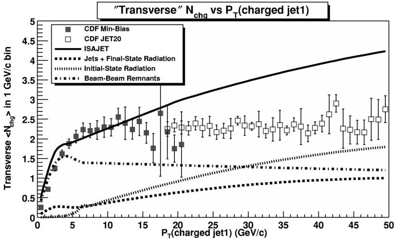
FIG. 32. Data from Fig. 21 on the average number of charged particles ( p_T > 0.5 GeV/c, |\eta| < 1 ) as a function of P_{T1} (leading charged jet) for the “transverse” region defined in Fig. 14 compared with the QCD Monte Carlo model predictions of ISAJET. The predictions of ISAJET are divided into three categories: charged particles that arise from the breakup of the beam particles (“beam-beam remnants”), charged particles that arise from initial-state radiation, and charged particles that result from the outgoing jets plus final-state radiation (see Fig. 1).
