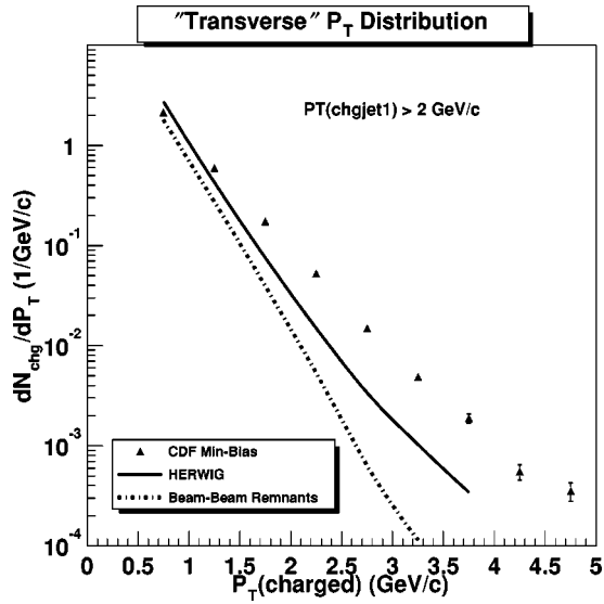
FIG. 38. Data from Fig. 37 on the transverse momentum distribution of charged particles ( p_T > 0.5 GeV/c, |\eta| < 1 ) in the “transverse” region defined in Fig. 14 for P_{T1} > 2 GeV/c compared to the QCD hard scattering Monte Carlo model predictions from HERWIG. The dashed curve shows the contribution arising from the breakup of the beam particles (“beam-beam remnants”) predicted by HERWIG.
