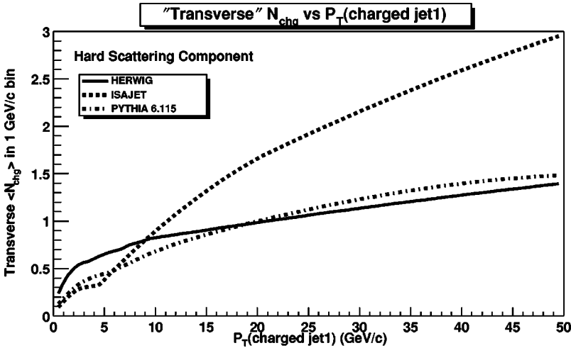
FIG. 35. QCD Monte Carlo model predictions from HERWIG, ISAJET, and PYTHIA 6.115 of the average number of charged particles ( p_T > 0.5 GeV/c, |\eta| < 1 ) as a function of P_{T1} (leading charged jet) for the “transverse” region defined in Fig. 14 arising from the outgoing jets plus initial and final-state radiation (“hard scattering component”).
