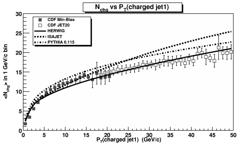
FIG. 13. The average number charged particles in the event ( p_T > 0.5 GeV/c, |\eta| < 1 , including chgjet1) as a function of the transverse momentum of the leading charged jet. The solid (open) points are the min-bias (JET20) data. The data are compared with the QCD Monte Carlo model predictions of HERWIG, ISAJET, and PYTHIA 6.115.
