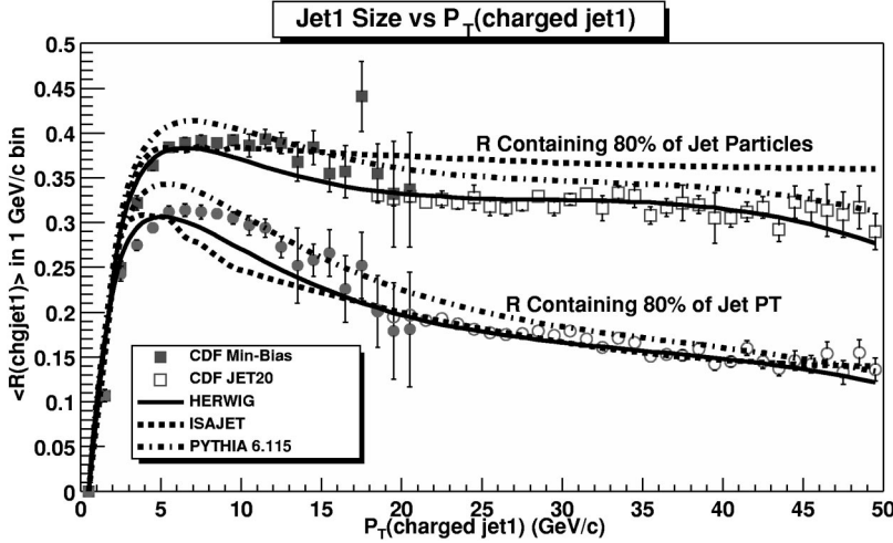
FIG. 6. The average radius in \eta - \phi space containing 80% of the charged particles (and 80% of the charged scalar p_T sum) as a function of the transverse momentum of the leading charged jet compared with the QCD Monte Carlo model predictions of HERWIG, ISAJET, and PYTHIA 6.115. The solid (open) points are min-bias (JET20) data.
