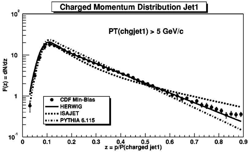
FIG. 11. Data from Fig. 10 on the momentum distribution of charged particles ( p_T > 0.5 GeV/c, |\eta| < 1 ) within chgjet1 (leading charged jet) for P_{T1} > 5 GeV/c compared with the QCD Monte Carlo model predictions of HERWIG, ISAJET, and PYTHIA 6.115.
