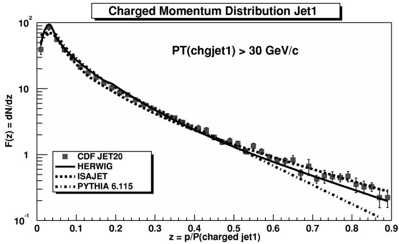
FIG. 12. Data from Fig. 10 on the momentum distribution of charged particles ( p_T > 0.5 GeV/c, |\eta| < 1 ) within chgjet1 (leading charged jet) for P_{T1} > 30 GeV/c compared with the QCD hard scattering Monte Carlo model predictions of HERWIG, ISAJET, and PYTHIA 6.115.
