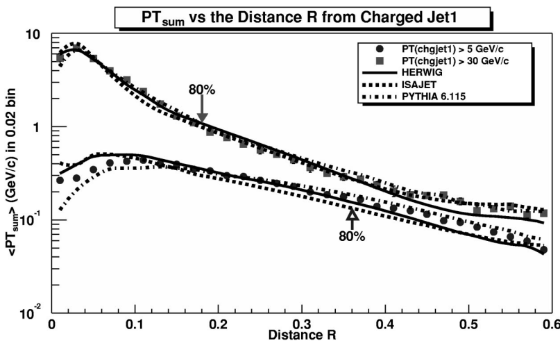
FIG. 9. Charged scalar p_T sum distribution in the radial distance R in \eta - \phi space from chgjet1 (leading charged jet) for charged particles with p_T > 0.5 GeV/c and |\eta| < 1 when P_{T1} > 5 GeV/c and 30 GeV/c. The points are \langle P_T \text{ sum} \rangle in a \Delta R = 0.02 bin (see Fig. 7). The P_{T1} > 5 GeV/c points are min-bias data and the P_{T1} > 30 GeV/c points are JET20 data. The data are compared with the QCD hard scattering Monte Carlo model predictions of HERWIG, ISAJET, and PYTHIA 6.115. For an average charged jet with P_{T1} > 5 GeV/c ( > 30 GeV/c), 80% of the jet p_T lies within R = 0.36 (0.18) as marked by the arrows.
