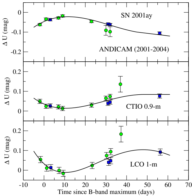
Figure 4. Similar to Figure 3, except these are U -band S -corrections for the unusual Type Ia SN 2001ay. The green dots correspond to corrections based on spectra with the Fred L. Whipple Observatory 1.5 m telescope. The blue squares correspond to corrections based on spectra with the MMT.
