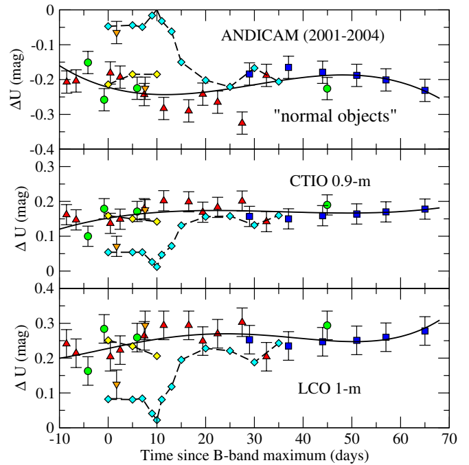
Figure 3. U -band S -corrections for “spectroscopically normal objects.” Symbols: red upward pointing triangles = SN 1999ee; blue squares = SN 2001el; green dots = SN 2002bo; and orange downward pointing triangles = SN 2004S. The top panel shows corrections for the ANDICAM instrument on the CTIO 1.3 m telescope. The middle panel shows corrections for the CTIO 0.9 m reflector. The bottom panel shows corrections for the Las Campanas Observatory 1 m telescope. The solid lines are low-order polynomial fits to these data. Connected by dashed lines we also show S -corrections based on Hsiao et al. (2007) templates warped to match the natural system magnitudes of SN 1999ee data from the CTIO 0.9 m telescope (cyan diamonds) and SN 2002bo data from ANDICAM when it was mounted on the Yale–AURA–Lisbon–Ohio (YALO) telescope at CTIO (yellow diamonds).
