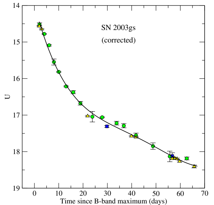
Figure 5. U -band photometry (with S -corrections) of SN 2003gs. There are now no significant systematic differences of photometry obtained with different telescopes.
