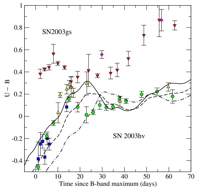
Figure 7. U-B color curves of SNe 2003hv and SN 2003gs. The photometry of SN 2003hv has been S -corrected and corrected for a small amount of Milky Way reddening ( E(U-B) = 0.011 ). Symbols: green dots (CTIO 1.3 m), blue squares (CTIO 0.9 m), and yellow upward pointing triangles (LCO 1 m). For SN 2003gs, E(U-B) = 0.025 mag, which has been subtracted out. Symbols: red downward pointing triangles (CTIO 1.3 m) and magenta diamonds (CTIO 0.9 m). The solid line is the MLCS2K2 locus for \Delta = +0.4 . The dashed line is for \Delta = 0.0 . The dot-dashed line is for \Delta = -0.4 .
