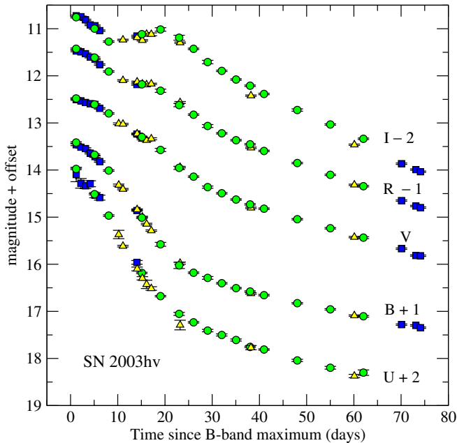
Figure 6. UBVR-I -band photometry (with S -corrections) of SN 2003hv. The CTIO 0.9 m and LCO 1 m BVR-I data (blue squares and yellow upward pointing triangles, respectively) are from Leloudas et al. (2009), with S -corrections provided by G. Leloudas. The CTIO 1.3 m data are plotted as green dots. We have excluded KAIT data and data from the Siding Spring Observatory 2.3 m.
