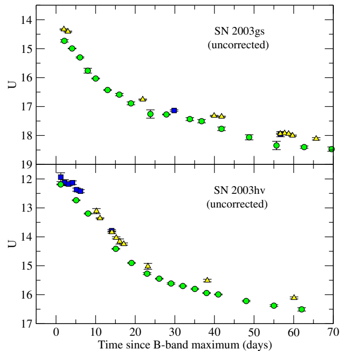
Figure 1. U -band photometry (without S -corrections) of SN 2003gs and SN 2003hv. Symbols: green circles = CTIO 1.3 m with ANDICAM; blue squares = CTIO 0.9 m; and yellow triangles = LCO 1 m.
