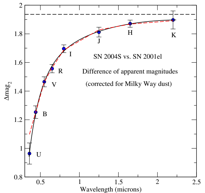
Figure 8. Difference of apparent magnitudes of SNe 2001el and 2004S, following Figure 14 of Krisciunas et al. (2007). The U -band difference is now based on S -corrected photometry. The horizontal dashed line is the derived difference of the distance moduli. The solid line is a fourth-order fit to the UBVRJHK points. The red dashed line is based on a distance modulus difference of 1.936 mag, A_V = 0.472 mag and scale factors A_\lambda/A_V from Table 6 of Krisciunas et al. (2007), using a CCM89 extinction law and R_V = 2.15 .
