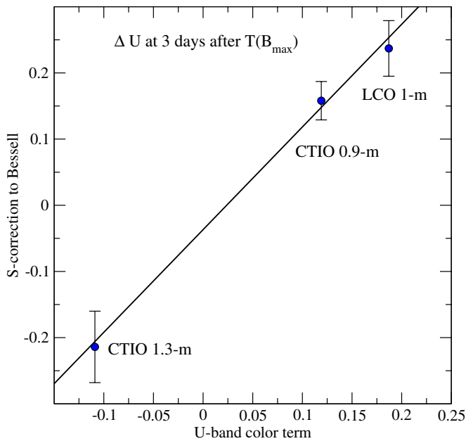
Figure 9. U -band S -correction as a function of U -band photometric color term. (A color version of this figure is available in the online journal.)
