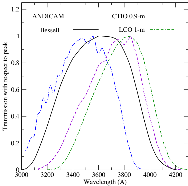
Figure 2. Effective U -band transmission functions of the cameras on the CTIO 1.3 m, CTIO 0.9 m, and LCO 1 m telescopes, along with the U -band filter specified by Bessell (1990).
