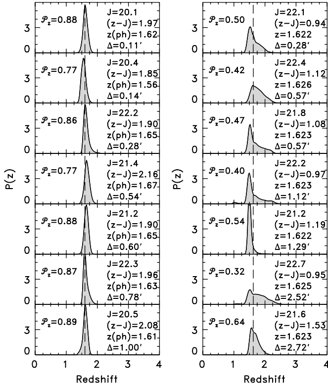
Figure 5. Photometric-redshift probability-distribution functions, P(z) , for galaxies in ClG J0218.3-0510. The left figure shows the P(z) for the seven galaxies that have integrated redshift probabilities, \mathcal{P}_z > 0.75 with angular separations of \Delta < 1' of the cluster center. Without exception, these galaxies all have very red (z - J) colors. Each panel gives the (z - J) color, J magnitude, the most likely photometric redshift, the integrated redshift probability, and angular separation from the cluster center. Although these galaxies lack spectroscopic information, their large integrated redshift probabilities support the assertion that they are at the cluster redshift, z = 1.62 , indicated by the vertical dashed lines. The cluster galaxies with spectroscopic redshifts all show [O II] in their spectra, implying ongoing star formation (see Figure 2). They have bluer (z - J) colors and lower values of \mathcal{P}_z , presumably because they have weaker 4000 Å/Balmer breaks owing to the star formation activity. The right figure shows the P(z) for the seven galaxies with spectroscopic redshifts 1.62 < z < 1.63 . Each panel shows the same information as for the left figure, except that they give the spectroscopic redshift instead of the most likely photometric redshift.
