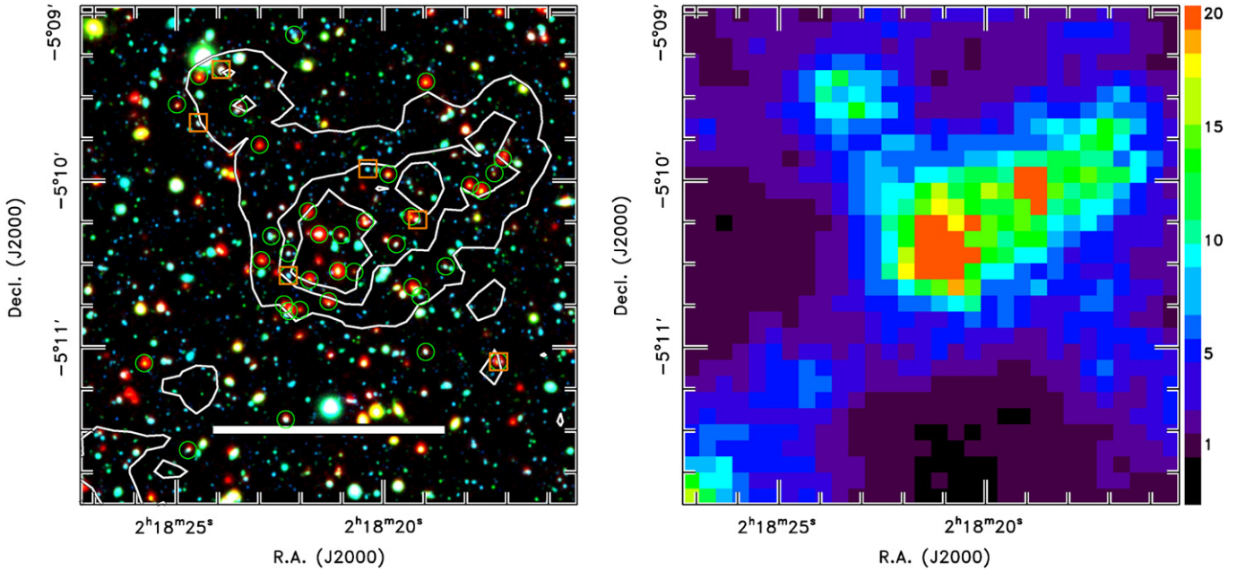
Figure 1. Left panel shows a false-color image of the target field. Blue corresponds to the Suprime-Cam B band, green to the Suprime-Cam i band, and red to the Spitzer 4.5 \mu\text{m} band. The images have not been corrected for variations in the data image quality. The image spans 3' \times 3' , corresponding to 1.5 \text{ Mpc} \times 1.5 \text{ Mpc} at z = 1.62 . The heavy white bar shows a distance of 0.7 Mpc at the redshift of the cluster. Small green circles denote candidate cluster members with \mathcal{P}_z > 0.5 as defined in Section 2.4. Orange squares denote those objects with spectroscopically confirmed redshifts 1.62 < z < 1.65 . The contours denote regions with 5 , 10 , and 15\sigma above the mean density of galaxies with 1.5 < z_{\text{phot}} < 1.7 . The right panel shows the surface density of galaxies with 1.5 < z_{\text{phot}} < 1.7 in units of the number of standard deviations ( \sigma ) above the mean density, ranging from -1 to 20 (as indicated in the plot legend).
