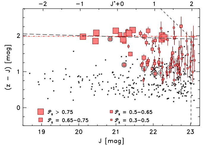
Figure 6. Color-magnitude diagram of all galaxies within \Delta < 2' of the cluster center, corresponding to 1 Mpc at z = 1.62 . The top axis shows magnitudes in units of J^* , the characteristic luminosity evolved from the measured values for the Coma cluster (de Propris et al. 1999) to z = 1.62 . The symbol size denotes that the galaxy lies at the cluster redshift based on the integrated redshift probability, \mathcal{P}_z , as indicated in the legend. The smallest gray squares all have \mathcal{P}_z < 0.3 , and are likely foreground or background field galaxies, unassociated with the cluster. Larger, red squares correspond to galaxies with \mathcal{P}_z > 0.3 , and likely associated with the cluster. The long-dashed line shows a fit to the red sequence (see Section 4). The red dot-dashed line shows the expected color of a stellar population observed at z = 1.62 formed in a short burst at z_f = 2.4 as described in the text. Circles denote those objects spectroscopically confirmed from 1.62 < z < 1.65 . These are bluer galaxies owing to the presence of [O II] emission, facilitating their spectroscopic identification (see Section 2.5). The X symbol shows an object with a spectroscopic redshift outside this range. The short dashed lines indicate the 5\sigma magnitude limits derived for point sources in the imaging data. A strong red sequence is apparent, which is dominated by galaxies with high \mathcal{P}_z .
