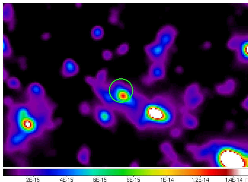
Figure 4. Summed XMM image centered on the position of CIG J0218.3-0510. CIG J0218.3-0510 is located on the edges of three adjacent XMM positions. The co-added XMM data yield an unambiguous source with 4\sigma significance in the [0.5–2.5] keV band within 10'' of the position of the cluster. The circle indicates the associated X-ray source and has a diameter of 40'' . The units of the color scale is \text{erg s}^{-1} \text{cm}^{-2} \text{arcmin}^{-2} as indicated by the running bar along the bottom of the image.
