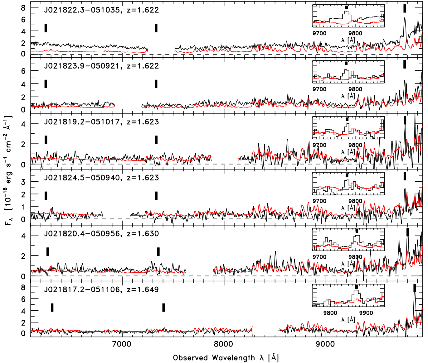
Figure 2. Extracted IMACS spectra for the six galaxies with 1.62 < z < 1.65 within 1/4 of the cluster center (corresponding to r < 0.7 Mpc at z = 1.62 ). The inset panel shows the region around [O II] \lambda 3727 at the measured redshift. In all panels, the black line is the measured spectrum. Gaps in the spectra show wavelengths that fall on the “gaps” between the IMACS CCDs. The red line shows the 1\sigma uncertainties propagated through the data reduction. The thick black lines show the expected locations of Fe II \lambda 2374 , Mg II \lambda 2800 , and [O II] \lambda 3727 for the measured redshift.
