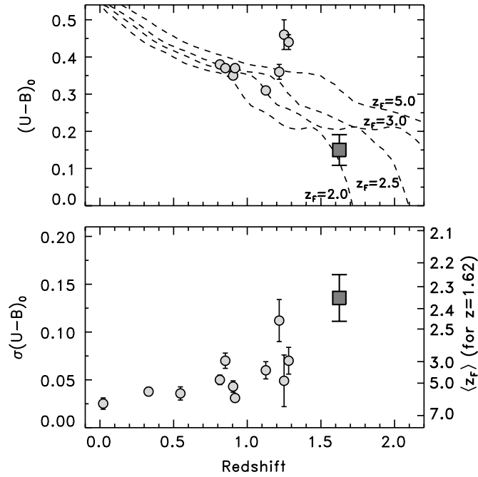
Figure 7. Top panel shows the evolution of the rest-frame U - B color measured at rest-frame M_B = -21.4 mag for red-sequence galaxies in clusters as a function of redshift. Smaller circles show the results from lower redshift clusters (Bower et al. 1992; Ellis et al. 1997; van Dokkum et al. 1998a, 1998b, 2000; Mei et al. 2009). The large box point shows the value derived for the cluster CIG J0218.3-0510 at 1.625 derived here. The curves show the expected evolution of a stellar population with solar metallicity formed with an e -folding timescale \tau = 0.1 Gyr at the formation redshift indicated. The bottom panel shows the evolution of the scatter in the rest-frame U - B color for red-sequence galaxies as a function of redshift. Symbols are the same as the top panel. The scatter in the colors of red-sequence galaxies increases with redshift. The right axis of the bottom panel indicates the expected scatter in the rest-frame (U - B) color for a red sequence observed at z = 1.62 for a given mean luminosity-weighted formation redshift (see the text). The scatter in the (U - B) color for the z = 1.62 cluster corresponds to a luminosity-weighted formation redshift of z_f = 2.25 – 2.45 , consistent with the evolution in the (U - B)_0 color.
