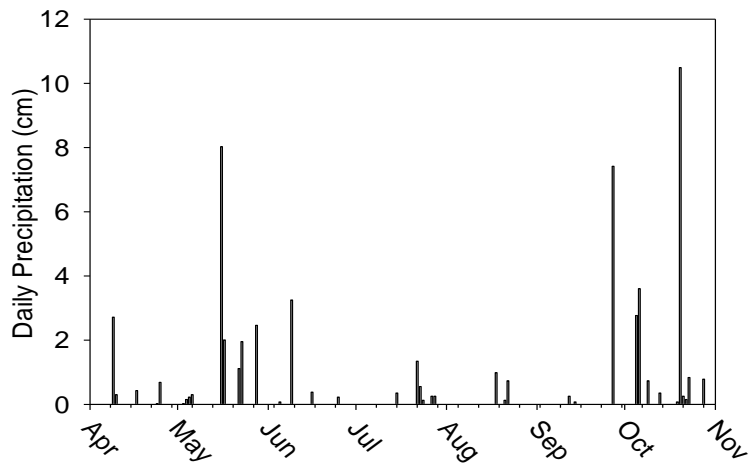
Figure 2.1. Daily percipitaion (cm) throughout the 2012 season. Data from the Texas ET network, Texas A&M Golf Course Weather Station.
