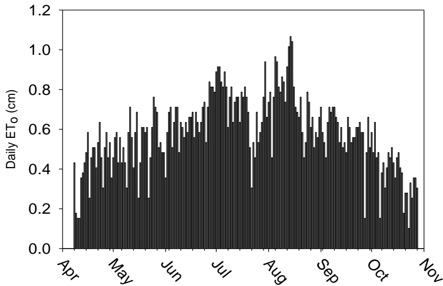
Figure 2.4. Daily ET 0 throughout the 2013 season. Data from the Texas ET network, Texas A&M Field Lab Weather Station.
