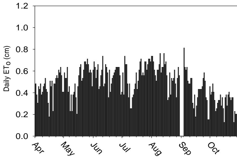
Figure 2.3. Daily ET 0 throughout the 2012 season. Data from the Texas ET network, Texas A&M Golf Course Weather Station.
