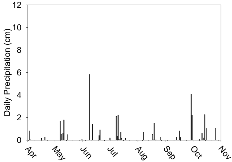
Figure 2.1. Daily percipitaion (cm) throughout the 2012 season. Data from the Texas ET network, Texas A&M Golf Course Weather Station.
