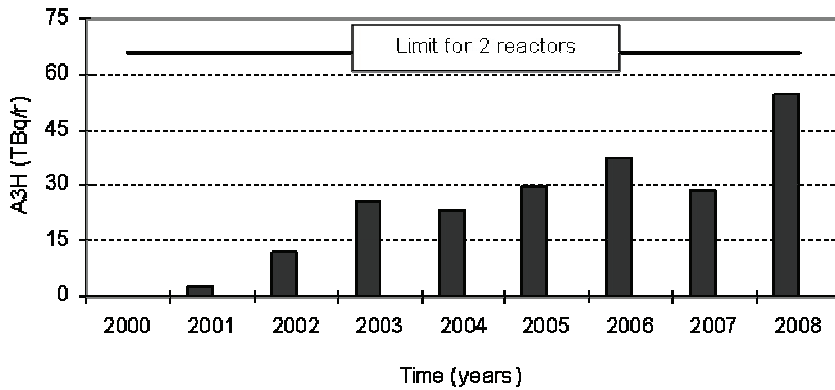
Fig. 4. Annual outflows of tritium discharged with waste water from Temelín Nuclear Power Plant in the period 2000 - 2008
