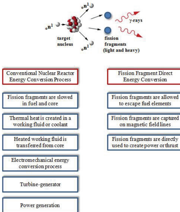
Fig. 1. Conventional nuclear reactor and direct energy conversion processes.
