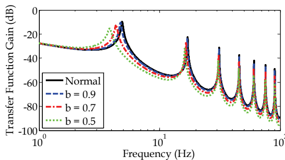
Fig. 9. Transfer functions of a pressure sensing system under normal condition and with sensing line blockages.
