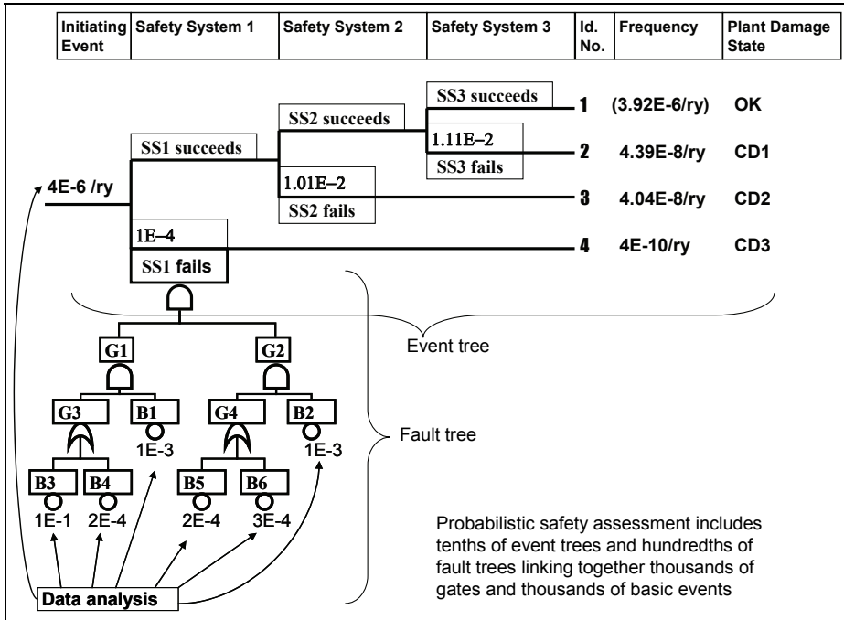
Fig. 3. Fault tree and event tree integration
