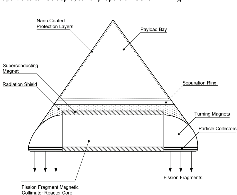
Fig. 4. Conceptual implementation of the FFMCR configuration.
