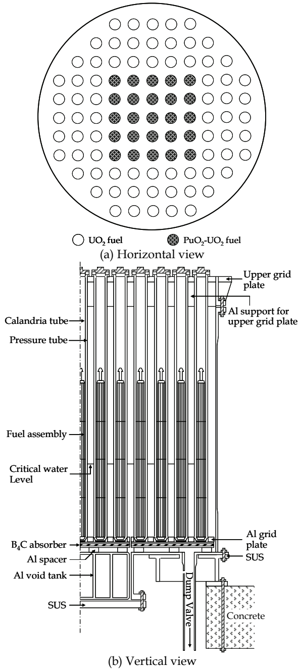
Fig. 1. Configuration of DCA core with a lattice pitch of 25 cm
