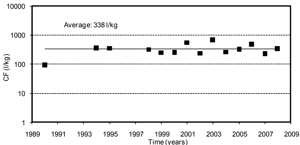
Fig. 12. 137 Cs concentrations factors in fish during the period 1990 – 2008
