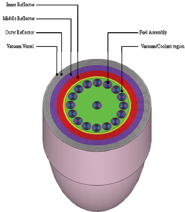
Fig. 2. Internal components of the FFMCR system.
