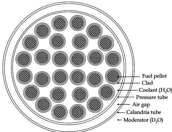
Fig. 2. Cross-sectional view of a 28-rod fuel assembly
