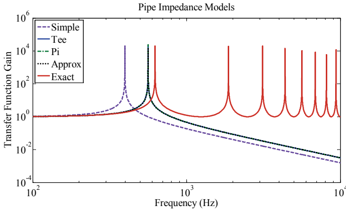
Fig. 5. Transfer functions for the exact ( \mathbf{H}_E ), pi and tee ( \mathbf{H}_G ), simple L ( \mathbf{H}_S ), and approximate ( \mathbf{H}_A ) pipeline models. The pi, tee and approximate models overlay one another. The pipe system parameters are \ell = 60 cm; r = 0.8 cm; \mu = 0.01 g/cm s; \rho = 1 g/cm 3 ; c = 150,000 cm/s; Re = 1000 ; and \bar{Q} = 6.25 cm/s.
