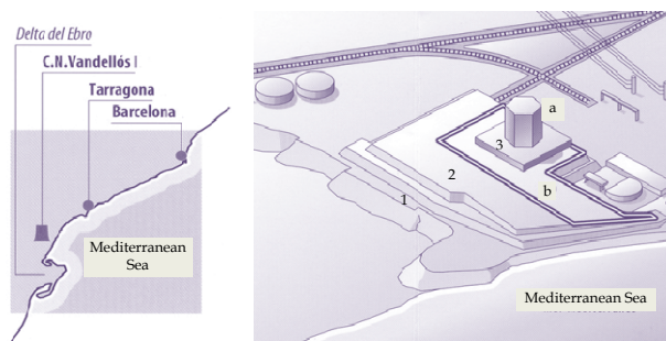
Fig. 2. Sketch with location (points 1 to 3) of corrosion stations
