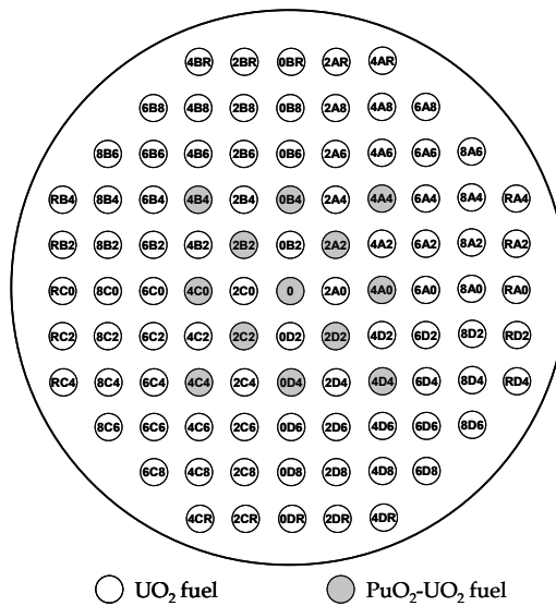
Fig. 3. Channel identification of a scattered DCA core
