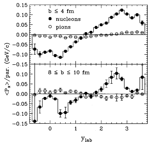
FIG. 1. The average transverse momentum of nucleons and pions in the central (upper window) and peripheral (lower window) collisions of Au+Au at p_{\text{beam}}/A=10.8 GeV/c.
