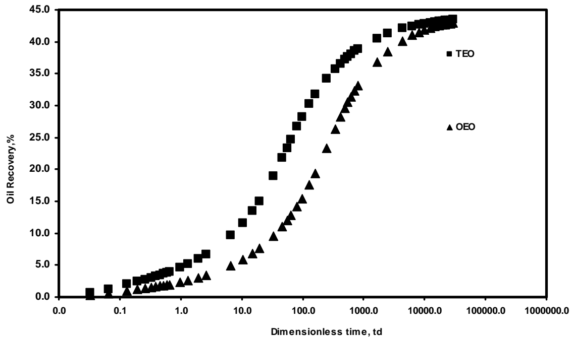
Fig 5.1 — Correlation of the results for the systems with different boundary conditions, using the length of the core in the equation of dimensionless time
