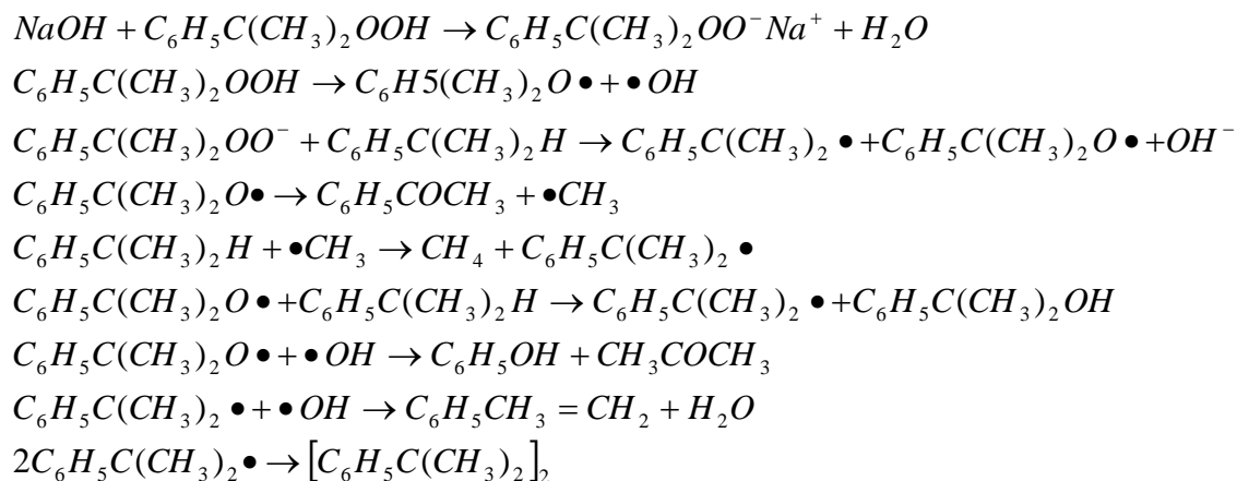
Figure 5 Scheme 2 for alkaline CHP decomposition reaction
