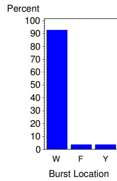
Histogram of Burst Location By Package Adhesive=Amcor Package=PS5
