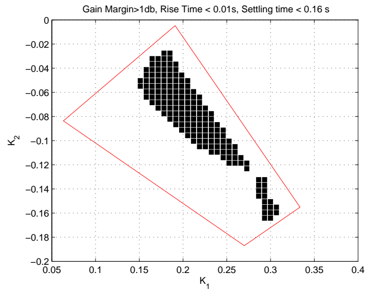
Fig. 26. Subset satisfying gain margin > 1db , rise time < 0.01s and settling time < 0.16s for the plant in example III.10
