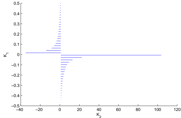
Fig. 3. Stabilizing set of PI controller for example III.3
