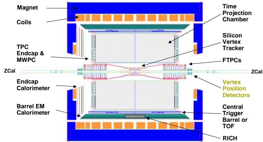
Fig. 3. The STAR detector
