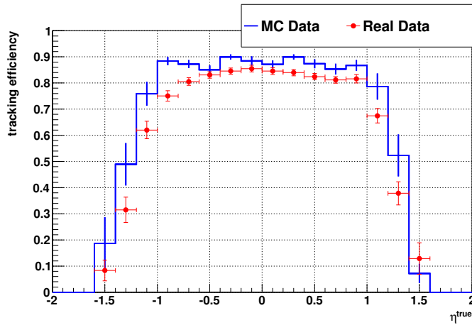
Fig. 18. Tracking efficiencies vs. pseudo-rapidity ( \eta ) of embedded tracks
