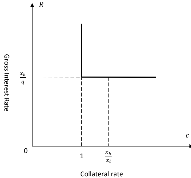
Fig. 10. \Omega when credit default swaps are allowed and \lambda^o = \frac{x_h}{q} , \lambda^p > 1 .
