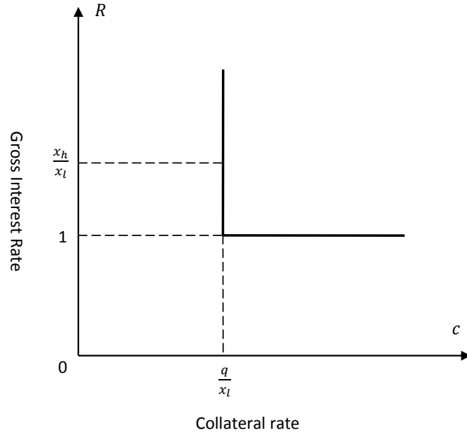
Fig. 11. \Omega when credit default swaps are allowed and \lambda^o > \frac{x_h}{q} , \lambda^p = 1 .
