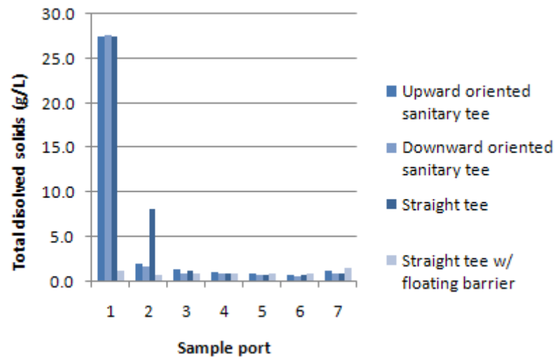
Figure 35. Comparison of the mean differences in initial and final total dissolved solids concentration in four downspout first flush diverters with a 10.16 cm diverter chamber at a flow rate of 75.71 L/min.
