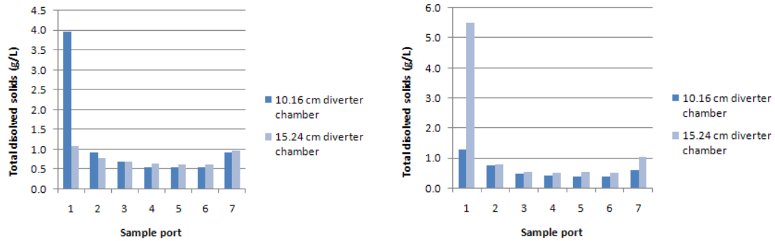
Figure 23. Comparison of the mean differences in initial and final total dissolved solids concentration in four downspout first flush diverters utilizing two downward oriented (left) and two upward oriented (right) sanitary tees at a flow rate of 3.03 L/min.
