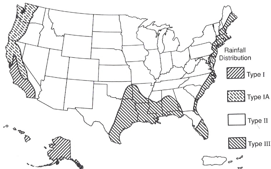
Figure 2. Applicable region for various SCS Type curves (Soil Conservation Service, 1986).
