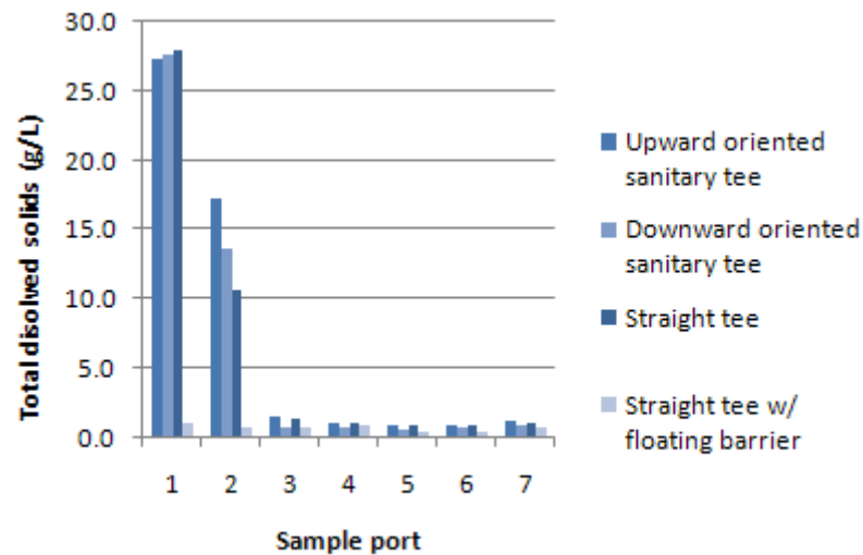
Figure 34. Comparison of the mean differences in initial and final total dissolved solids concentration in four downspout first flush diverters with a 10.16 cm diverter chamber at a flow rate of 43.91 L/min.
