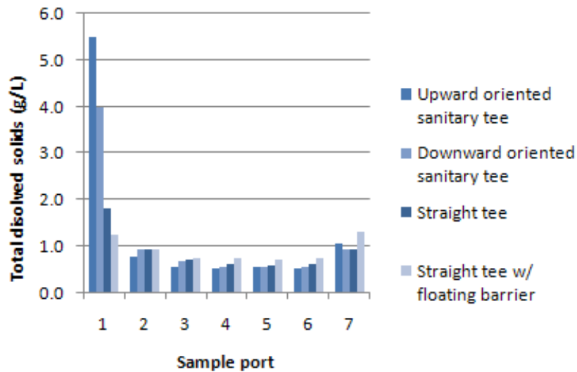
Figure 31. Comparison of the mean differences in initial and final total dissolved solids concentration in four downspout first flush diverters with a 10.16 cm diverter chamber at a flow rate of 3.03 L/min.
