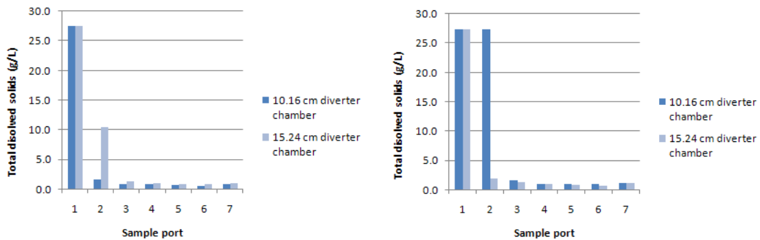
Figure 27. Comparison of the mean differences in initial and final total dissolved solids concentration in four downspout first flush diverters utilizing two downward oriented (left) and two upward oriented (right) sanitary tees at a flow rate of 75.71 L/min.
