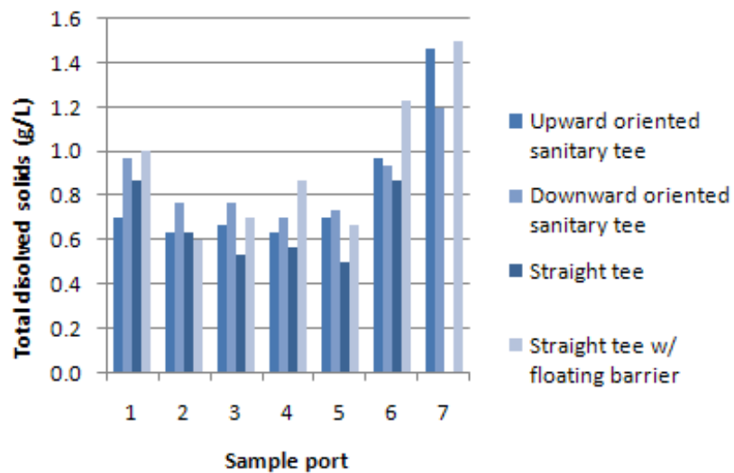
Figure 29. Comparison of the mean differences in initial and final total dissolved solids concentration in four downspout first flush diverters with a 10.16 cm diverter chamber at a flow rate of 0.76 L/min.
