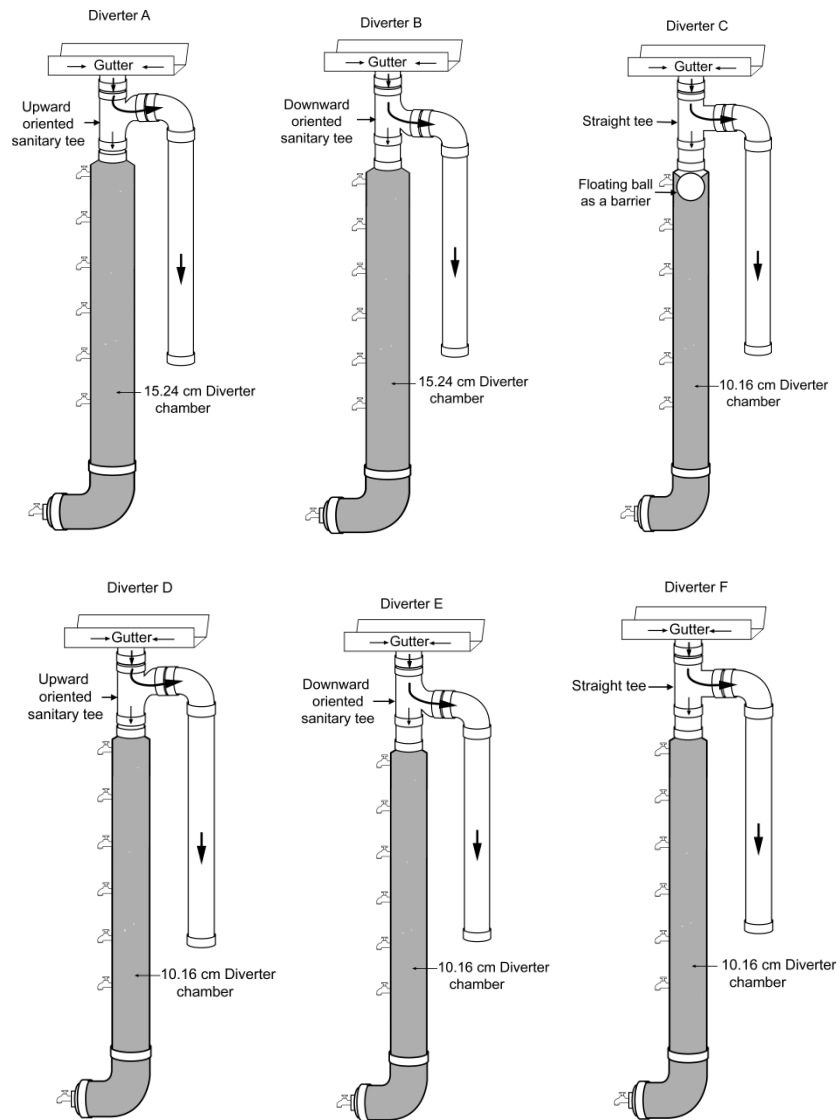
Figure 4. Six downspout first flush diverter configurations utilized for experiments.
