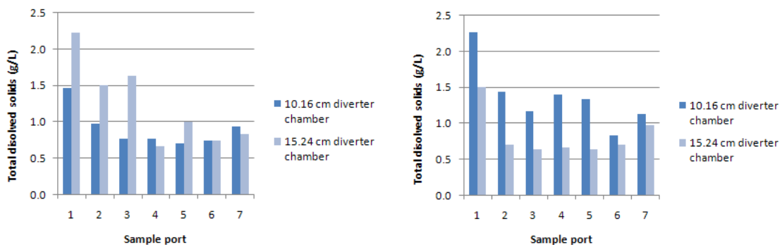
Figure 21. Comparison of the mean differences in initial and final total dissolved solids concentration in four downspout first flush diverters utilizing two downward oriented (left) and two upward oriented (right) sanitary tees at a flow rate of 0.76 L/min.
