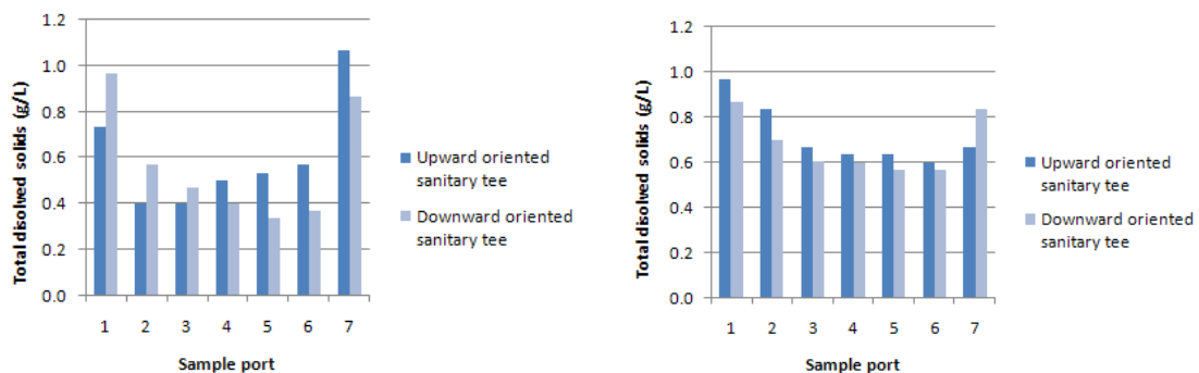
Figure 14. Comparison of the mean differences in initial and final total dissolved solids concentration in two 10.16 cm (left) and two 15.24 cm (right) diverter chambers at a flow rate of 1.51 L/min.
