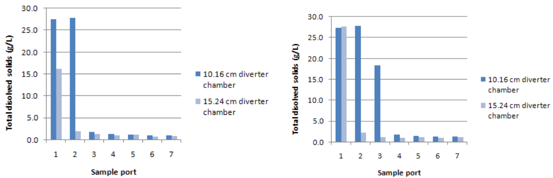
Figure 28. Comparison of the mean differences in initial and final total dissolved solids concentration four downspout first flush diverters utilizing two downward oriented (left) and two upward oriented (right) sanitary tees at a flow rate of 113.56 L/min.
