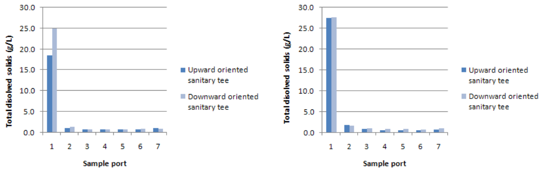
Figure 17. Comparison of the mean differences in initial and final total dissolved solids concentration in two 10.16 cm (left) and two 15.24 cm (right) diverter chambers at a flow rate of 22.71 L/min.
