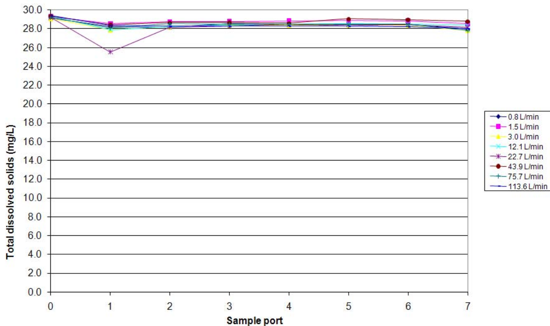
Figure 9. Diverter C's relationship between the mean total dissolved solids concentration and location of sampling ports in the diverter chamber at various flow rates with a closed diverter chamber drain.
