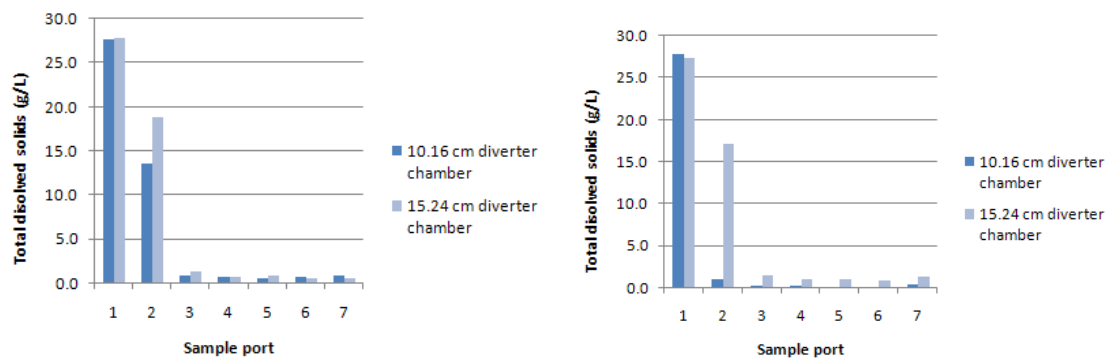
Figure 26. Comparison of the mean differences in initial and final total dissolved solids concentration in four downspout first flush diverters utilizing two downward oriented (left) and two upward oriented (right) sanitary tees at a flow rate of 43.91 L/min.
