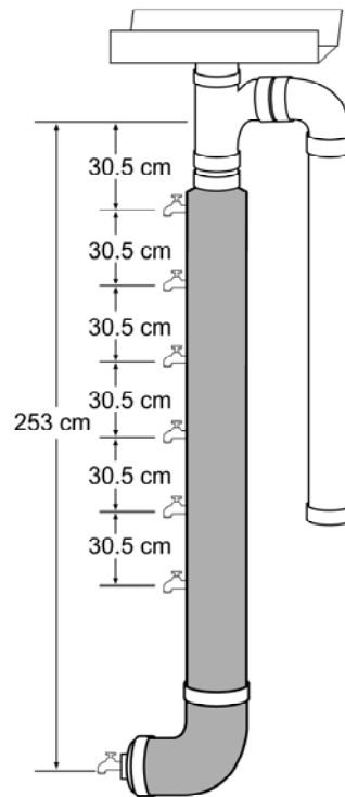
Figure 5. Diverter chamber sampling port locations relative to the diverter chamber to downspout transition fitting.
