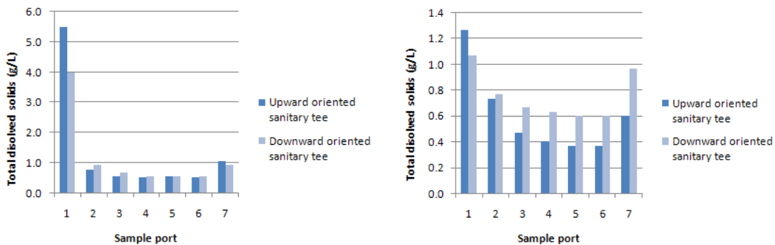
Figure 15. Comparison of the mean differences in initial and final total dissolved solids concentration in two 10.16 cm (left) and two 15.24 cm (right) diverter chambers at a flow rate of 3.03 L/min.
