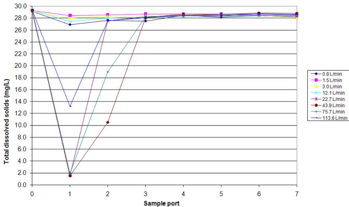
Figure 8. Diverter B's relationship between the mean total dissolved solids concentration and location of sampling ports in the diverter chamber at various flow rates with a closed diverter chamber drain.
