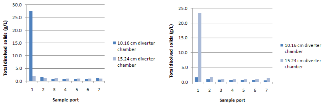
Figure 24. Comparison of the mean differences in initial and final total dissolved solids concentration four downspout first flush diverters utilizing two downward oriented (left) and two upward oriented (right) sanitary tees at a flow rate of 12.11 L/min.
