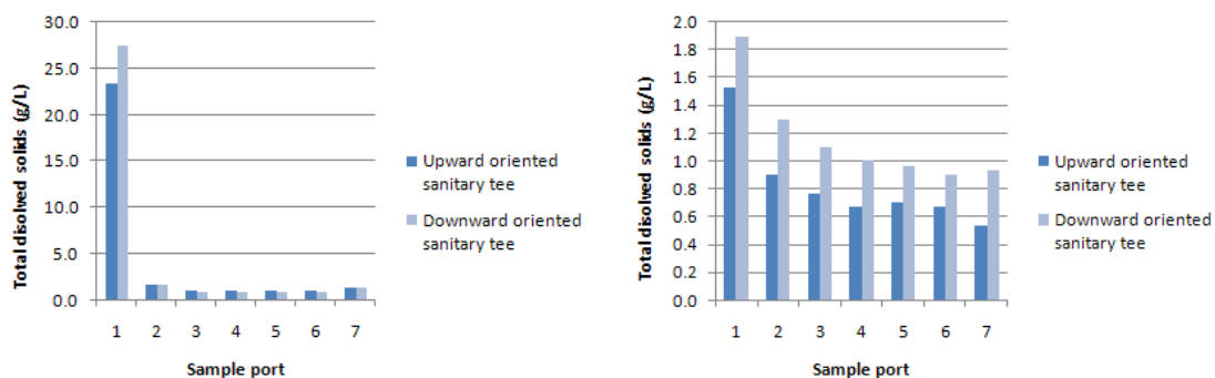
Figure 16. Comparison of the mean differences in initial and final total dissolved solids concentration in two 10.16 cm (left) and two 15.24 cm (right) diverter chambers at a flow rate of 12.11 L/min.
