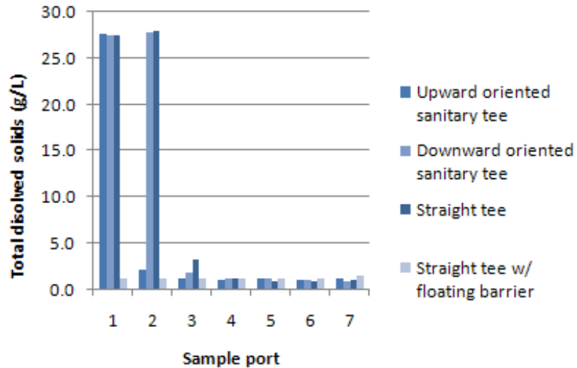
Figure 36. Comparison of the mean differences in initial and final total dissolved solids concentration in four downspout first flush diverters with a 10.16 cm diverter chamber at a flow rate of 113.56 L/min.
