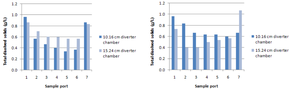
Figure 22. Comparison of the mean differences in initial and final total dissolved solids concentration in four downspout first flush diverters utilizing two downward oriented (left) and two upward oriented (right) sanitary tees at a flow rate of 1.51 L/min.
