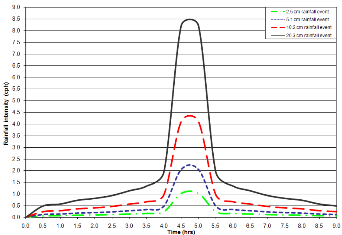
Figure 6. 2.5, 5.1, 10.2, and 20.3 cm SCS storm curve generated storm events for Austin, Texas.
