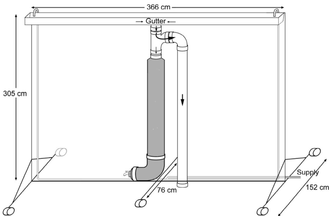
Figure 3. Downspout first flush diverter mounted on the test stand.
