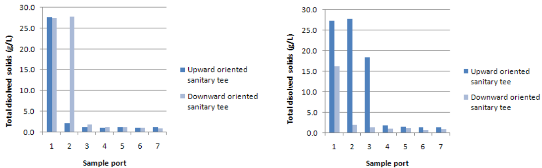
Figure 20. Comparison of the mean differences in initial and final total dissolved solids concentration in two 10.16 cm (left) and two 15.24 cm (right) diverter chambers at a flow rate of 113.56 L/min.
