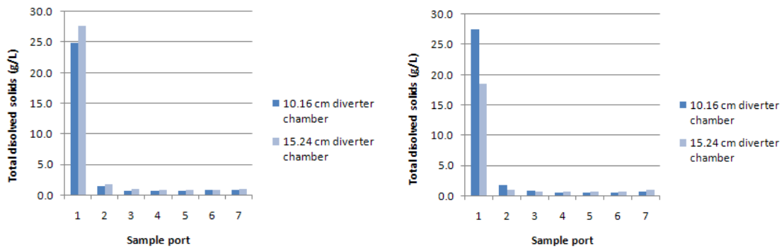
Figure 25. Comparison of the mean differences in initial and final total dissolved solids concentration in four downspout first flush diverters utilizing two downward oriented (left) and two upward oriented (right) sanitary tees at a flow rate of 22.71 L/min.
