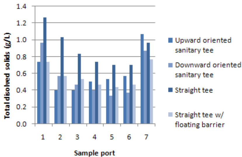
Figure 30. Comparison of the mean differences in initial and final total dissolved solids concentration in four downspout first flush diverters with a 10.16 cm diverter chamber at a flow rate of 1.51 L/min.
