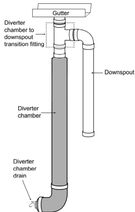
Figure 1. Diagram and basic components of a downspout first flush diverter.
