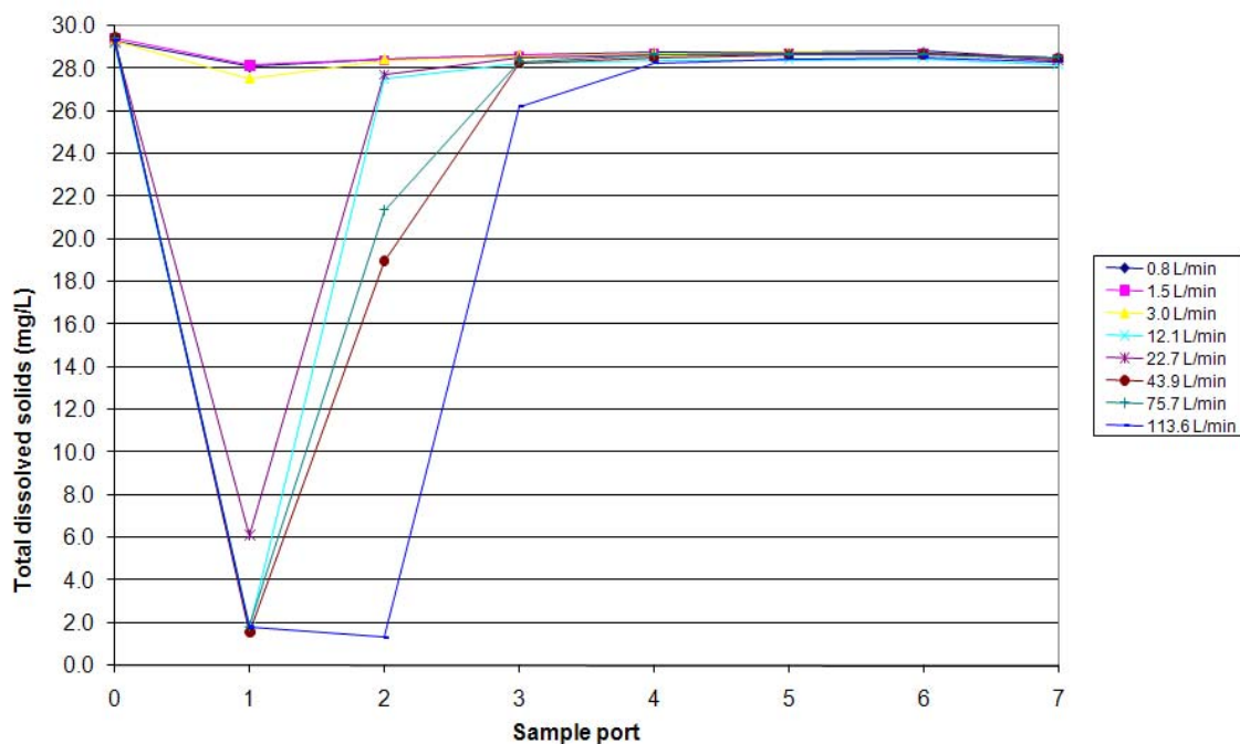
Figure 12. Diverter F's relationship between the mean total dissolved solids concentration and location of sampling ports in the diverter chamber at various flow rates with a closed diverter chamber drain.
