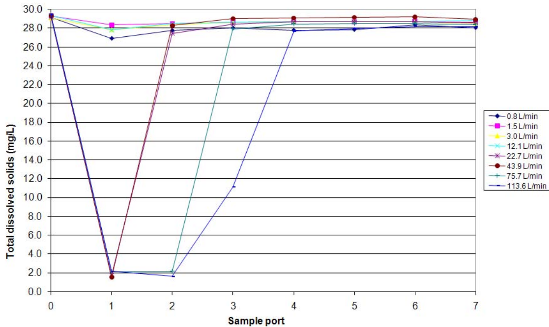
Figure 7. Diverter A's relationship between the mean total dissolved solids concentration and location of sampling ports in the diverter chamber at various flow rates with a closed diverter chamber drain.
