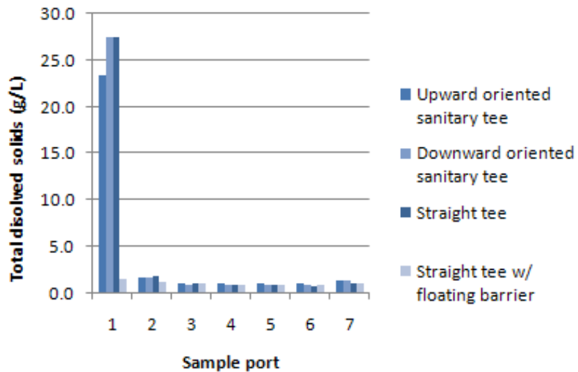
Figure 32. Comparison of the mean differences in initial and final total dissolved solids concentration in four downspout first flush diverters with a 10.16 cm diverter chamber at a flow rate of 12.11 L/min.
