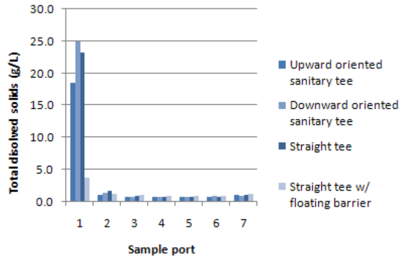
Figure 33. Comparison of the mean differences in initial and final total dissolved solids concentration in four downspout first flush diverters with a 10.16 cm diverter chamber at a flow rate of 22.71 L/min.
