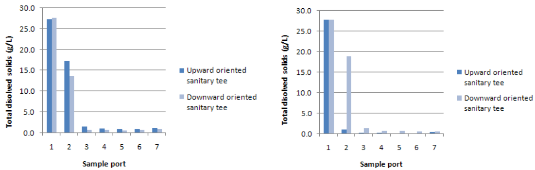
Figure 18. Comparison of the mean differences in initial and final total dissolved solids concentration in two 10.16 cm (left) and two 15.24 cm (right) diverter chambers at a flow rate of 43.91 L/min.
