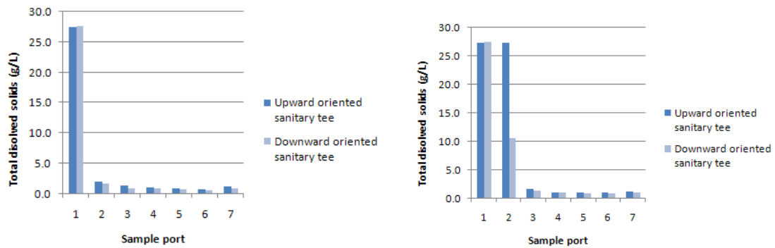
Figure 19. Comparison of the mean differences in initial and final total dissolved solids concentration in two 10.16 cm (left) and two 15.24 cm (right) diverter chambers at a flow rate of 75.71 L/min.
