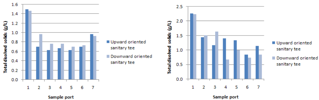
Figure 13. Comparison of the mean differences in initial and final total dissolved solids concentration in two 10.16 cm (left) and two 15.24 cm (right) diverter chambers at a flow rate of 0.76 L/min.
