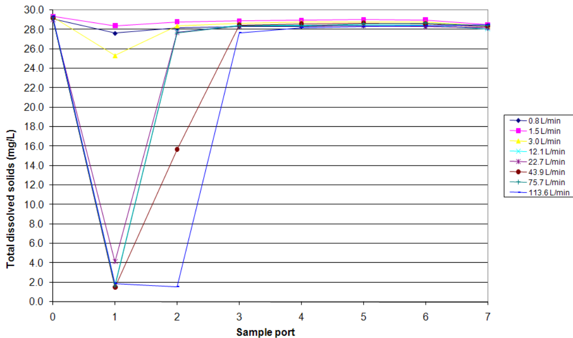
Figure 11. Diverter E's relationship between the mean total dissolved solids concentration and location of sampling ports in the diverter chamber at various flow rates with a closed diverter chamber drain.
