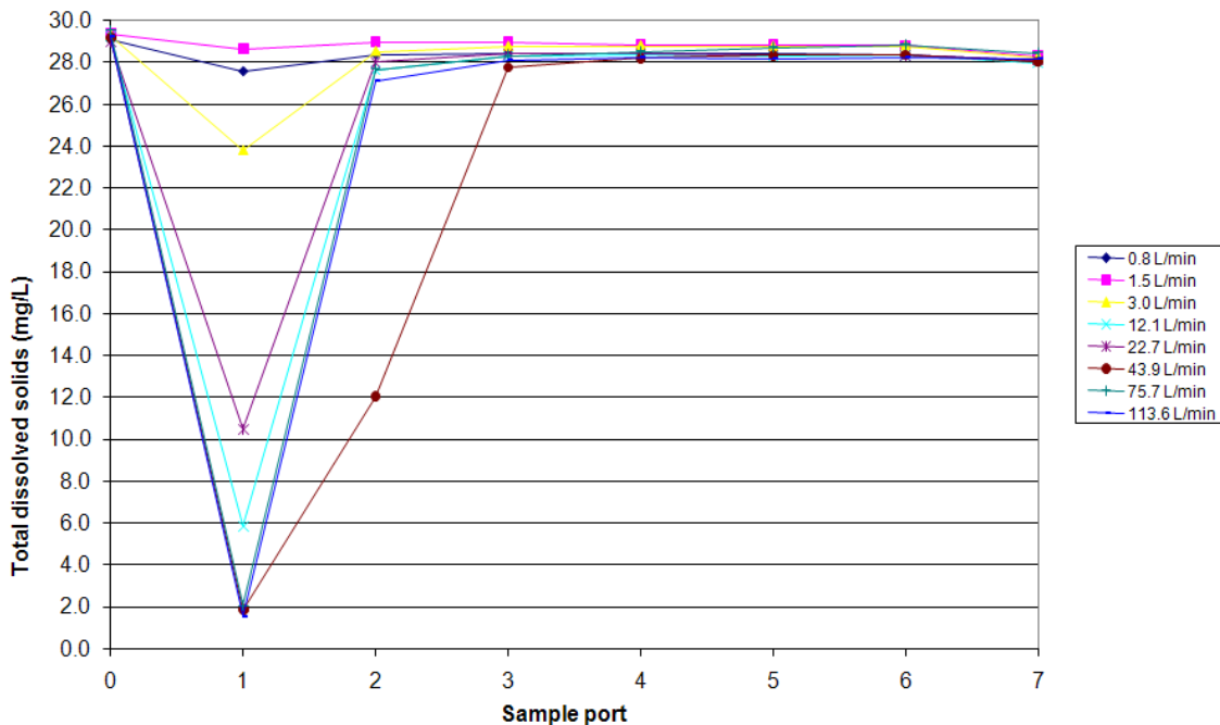
Figure 10. Diverter D's relationship between the mean total dissolved solids concentration and location of sampling ports in the diverter chamber at various flow rates with a closed diverter drain.
