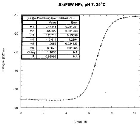
Fig. 3. Urea induced unfolding of BstF6W HPr in 10 mM sodium phosphate buffer, pH 7.0 at 25°C measured by CD absorbance at 222 nm. The solid line is fit to the data.
