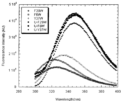
Fig. 2. Fluorescence emission scans for Bst F6W, F29W, and Y37W HPr. Open data points designate folded protein and closed data points designate unfolded protein. Protein denatured in 10.3 M urea, 10 mM sodium phosphate buffer, pH 7.0. Fluorescence signal was detected with a \lambda_{ex} of 280 nm.
