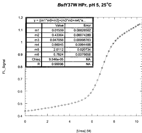
Fig. 8. Urea induced unfolding of BsfY37W HPr in 10 mM sodium phosphate buffer, pH 5.0. Fluorescence signal was detected using a 350 nm cut-off filter. The \lambda_{ex} was 280 nm.
