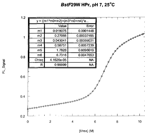
Fig. 7. Urea induced unfolding of BstF29W HPr in 10 mM sodium phosphate buffer, pH 7.0. Fluorescence signal was detected using a 350 nm cut-off filter. The \lambda_{ex} was 280 nm.
