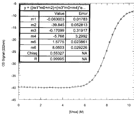
Fig. 5. Urea induced unfolding of BsfY37W HPr in 10 mM sodium phosphate buffer, pH 7.0 at 25°C measured by CD absorbance at 222 nm. The solid line is fit to the data.
