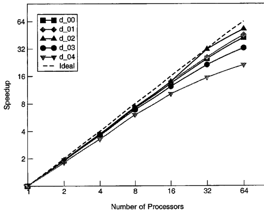
Deformation Test of ModifiedDCSC on ASCI Red 60 Angles Checked (Fixed size problem)
