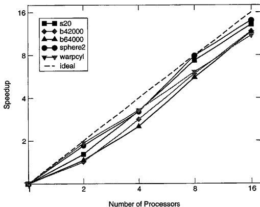
Fig. 11. Scalability of ModifiedDCSC on HP-V2200 for various meshes. This graph shows the scalability of ModifiedDCSC searching the DDGs of several meshes of different geometries.
