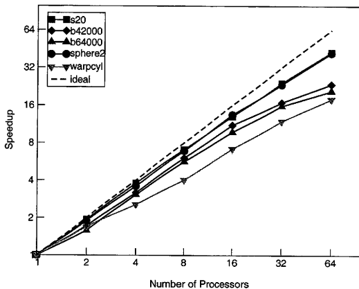
Fig. 12. Scalability of ModifiedDCSC on ASCI Red for various meshes. This graph shows the scalability of ModifiedDCSC searching the DDGs of several meshes of different geometries.
