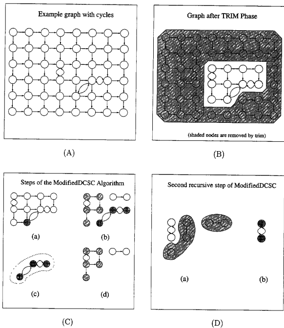
Fig. 5. ModifiedDCSC applied to an example graph.
