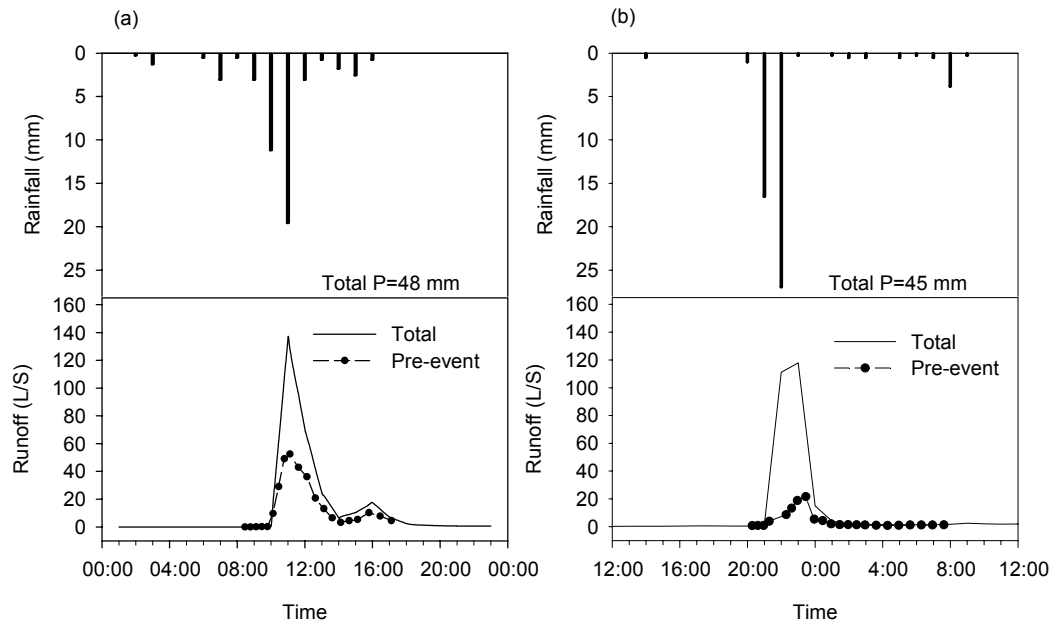
Figure 6. O-18 isotope hydrograph separation. (a) a winter event (20 February 2003) and (b) a summer event (27 June 2004).
