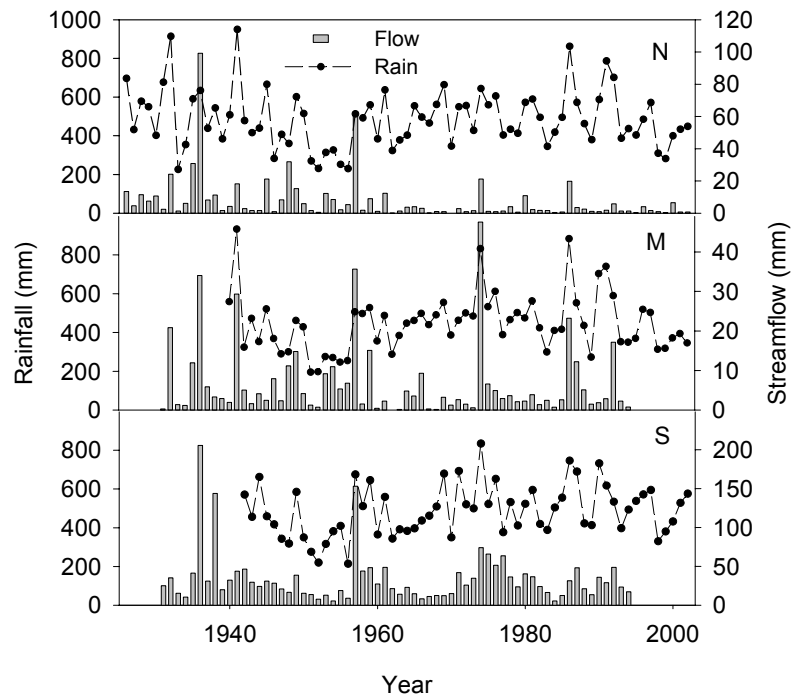
Figure 25. Annual total streamflow and precipitation in North, Middle and South Concho River basins. Basin-wide precipitation is obtained using Thiessen polygon method. Annual streamflow data reflects USGS Carlsbad, Tankersley and Christoval gauging station for North, Middle, and South Concho, respectively.
