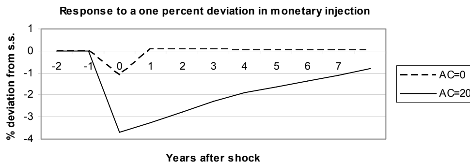
Figure 5.6: Consumption dynamics following a monetary shock
