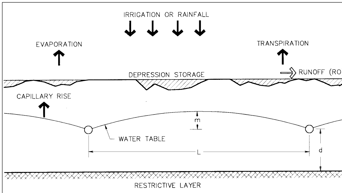
Figure 2. A subsurface drainage system. Plastic draitubes are located a distance ( L ) apart.
