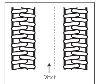
Figure 7. Pack the soil with a tractor tire on each side of the ditch.
