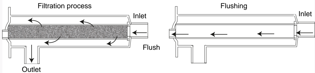
Fig. 6. Screen filter.
