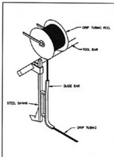
Figure V-5. Installation device commonly mounted on a tractor for burying drip strip tubing.
