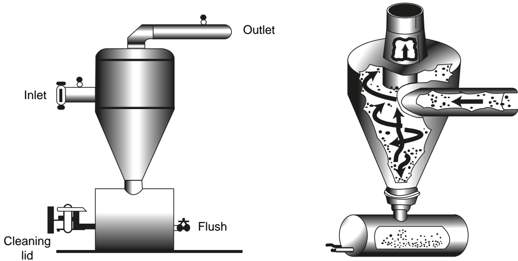
Fig. 5. Sand separator (centrifugal) filter.
