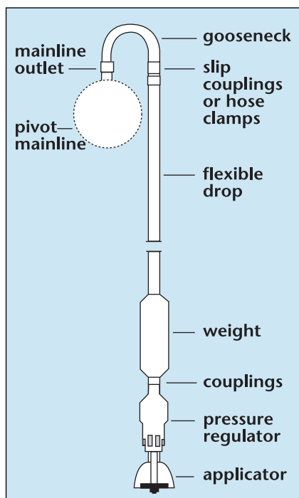
Figure 5. Drop arrangement.
