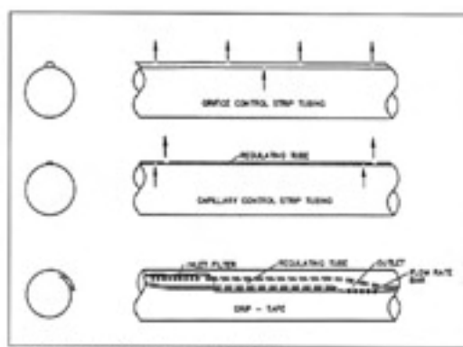
Figure V.4. Flow control design of common drip strip tubing.
