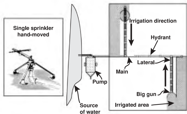
Figure 6. Big gun (left) and changing positions with two big gun sprinklers (right).
