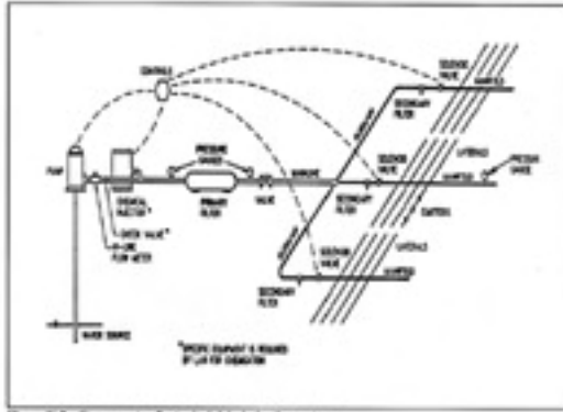
Figure V.2. Components of a typical drip irrigation system.
