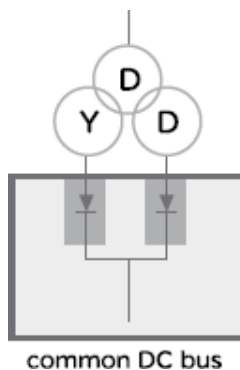
Figure 12. Multi-pulse arrangement
