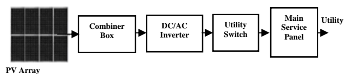
Figure 1. Simple PV System Diagram
