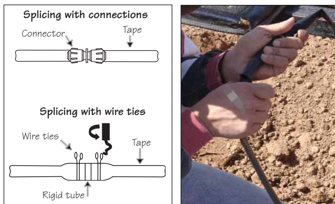
Figure 6. Drip line splicing.
