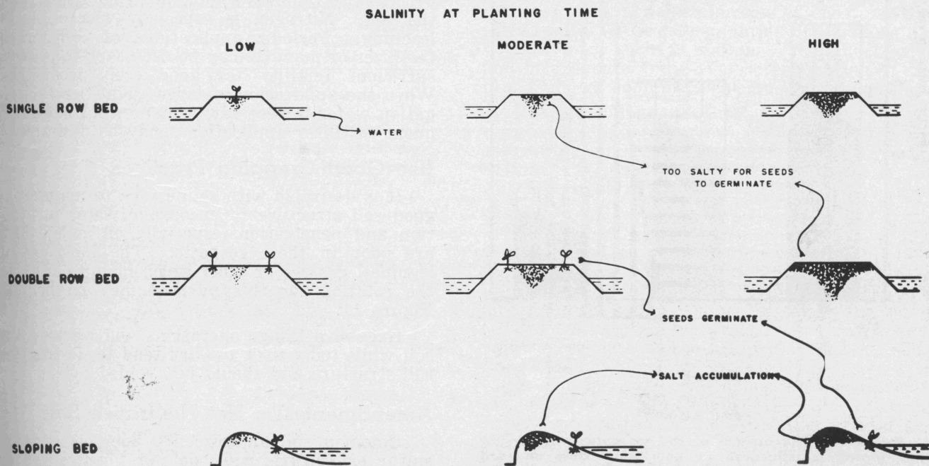
Figure 8. Effect of soil salinity and bed type on salt accumulation in a seeded area. Germination is delayed or prevented where salt accumulation is excessive.
