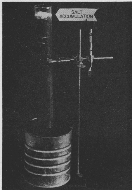
Figure 4. Saline soils often result from a high water table. Water will rise 4 to 6 feet or more in the soil above a free water surface. A salt deposit is left at the surface when water evaporates.
