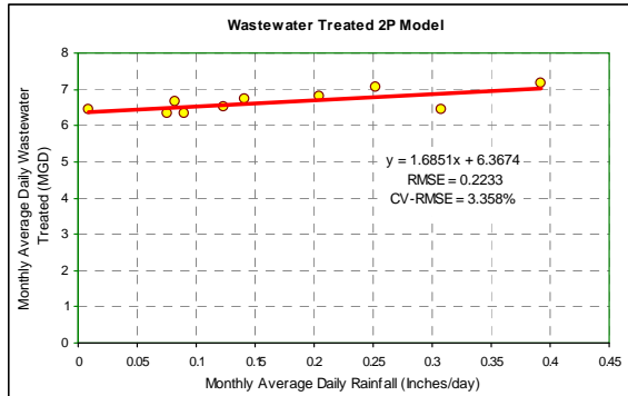
Figure 4. Monthly Average Daily Wastewater Treated versus Rainfall
