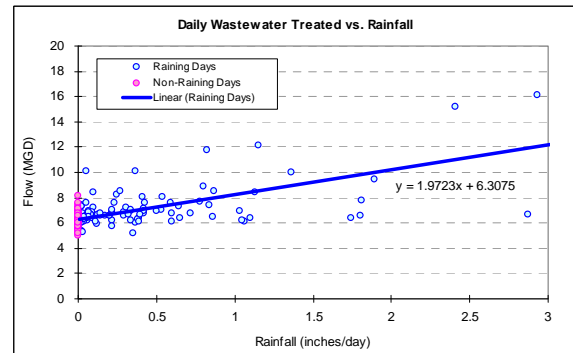
Figure 3. Daily Wastewater Treated versus Rainfall
