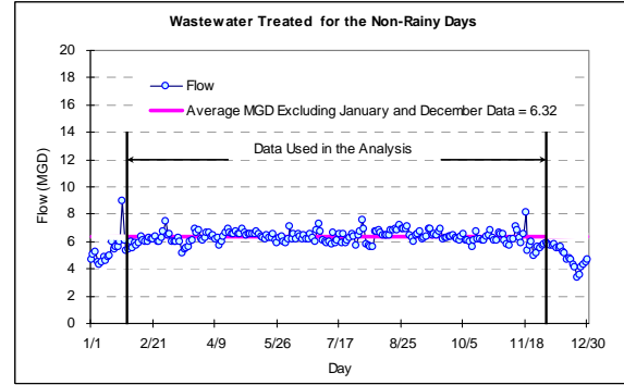
Figure 2. Wastewater Treated for the Non-Rainy Days
