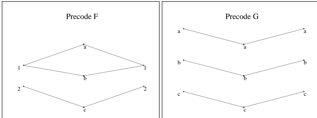
FIGURE 26. The Parametrization Given by Algorithm 8.5 (Example 8.18)
