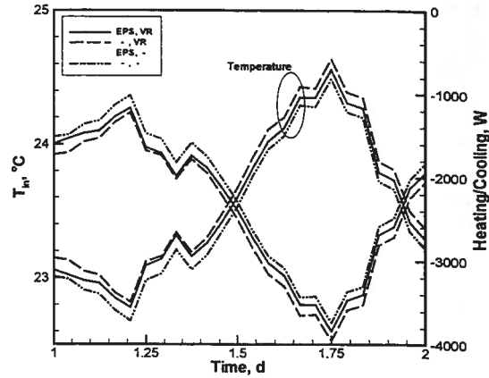
Figure 10. Indoor air temperature and heating/cooling
