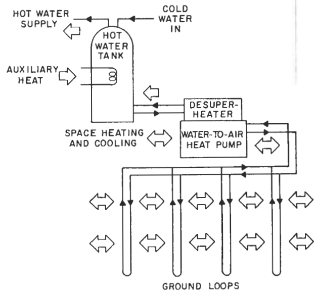
Figure 3. Ground-coupled heat pump with desuperheater.
