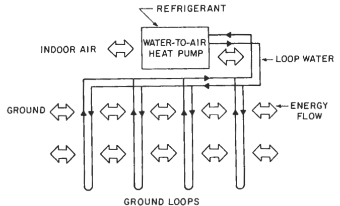
Figure 2. Ground-coupled heat pump.
