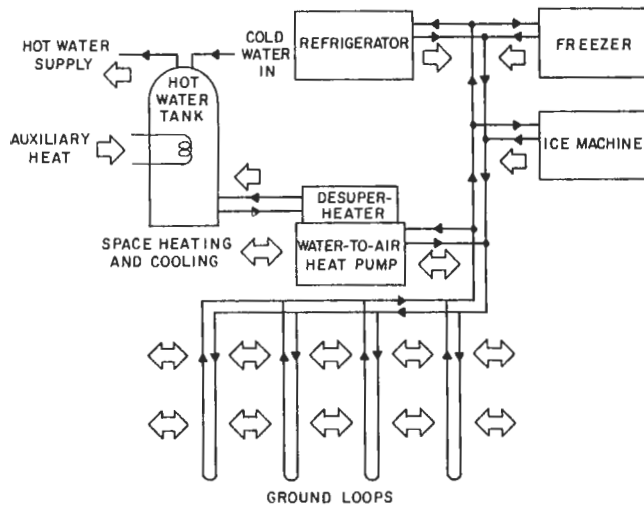
Figure 4. Ground-coupled heat pump and refrigeration.
