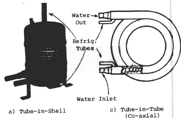
Figure 1. Water-to-Refrigerant Heat Exchangers
