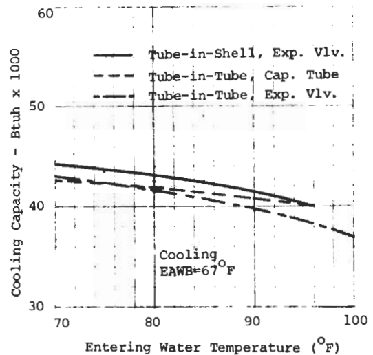
Figure 3. Heating and Cooling Capacities of Three Water-to-Air Heat Pumps
