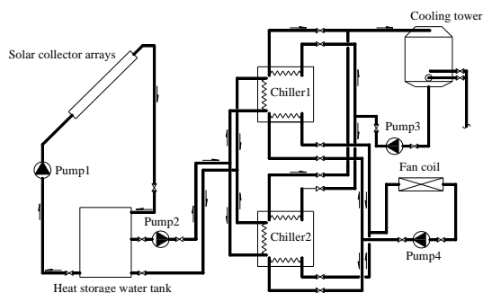
Fig.2 Flow diagram of solar-powered air-conditioning system
