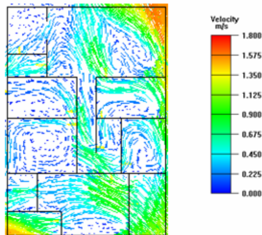
Fig.5 Velocity field across Y=1.5m in the middle apartment
