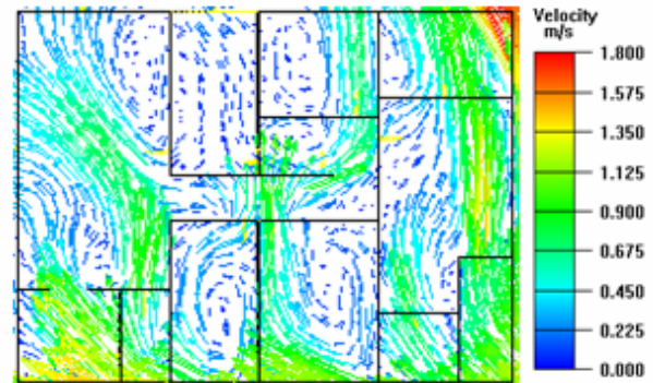
Fig.4 Velocity field across Y=1.5m in the east apartment
