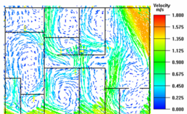
Fig.6 Velocity field across Y=1.5m in the west apartment
