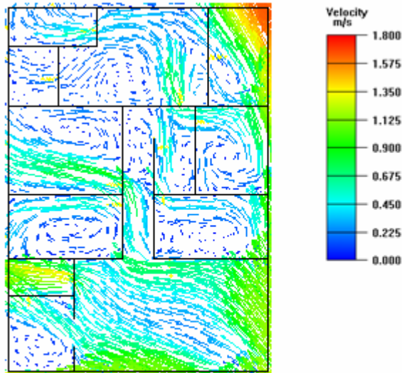
Fig.7 Velocity field across Y=1.5m in the north apartment
