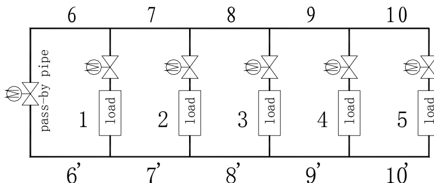
Fig.2 Map of air conditioning water system
