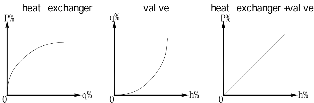
Fig.1 Relationship between heat quantity exchanged and valve opening
