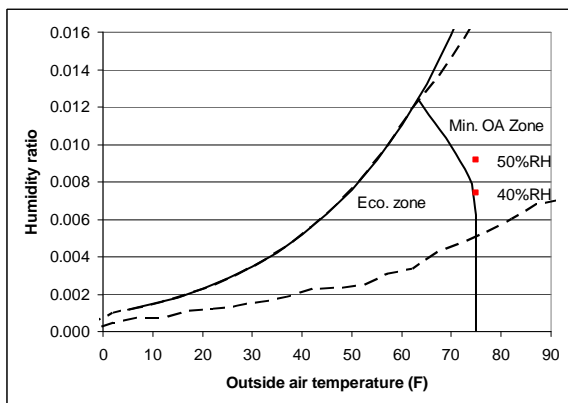
(a) No indoor humidity control
