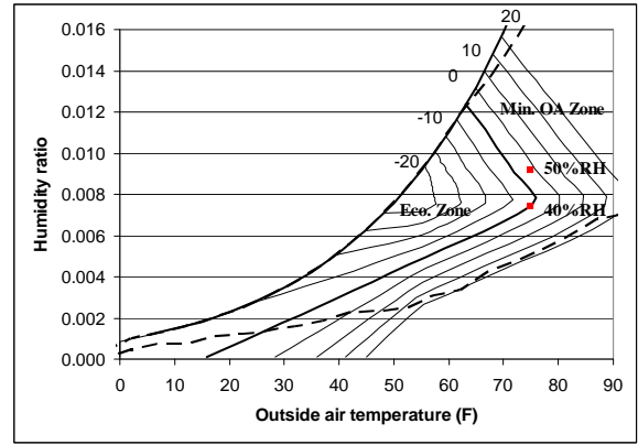
(9) Energy price ratio of 2.0 and 40% humidity
