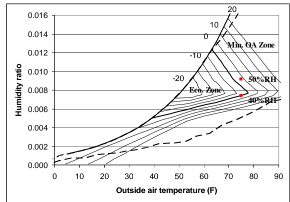
(10) Energy price ratio of 4.0 and 40% humidity
