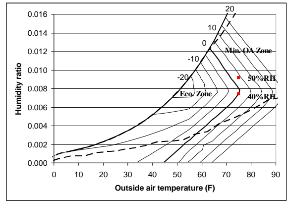
(8) Energy price ratio of 1.0 and 40% humidity
