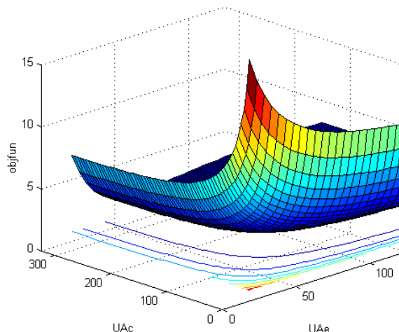
Figure 2. Objective function – Laboratory Chiller
