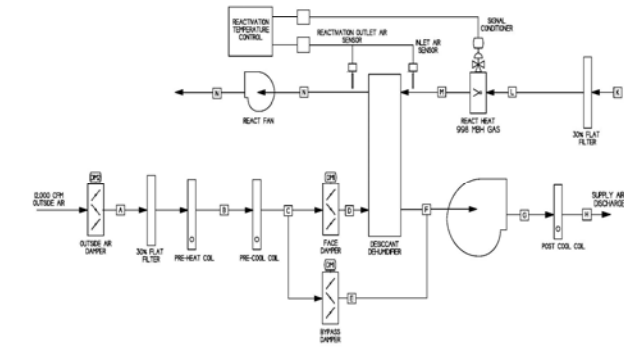
Figure 3: Flow schematic and operating conditions of the desiccant dehumidification unit.
