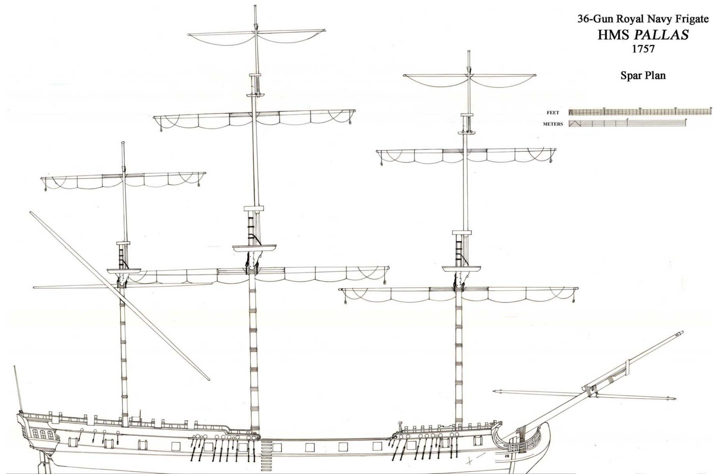
Fig. 30. Spar plan for frigate HMS Pallas .
