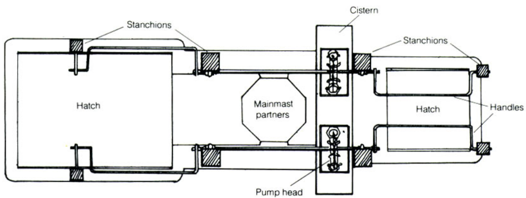
Fig. 26. Overhead view of chain-pump, Lavery, 1987, 71
