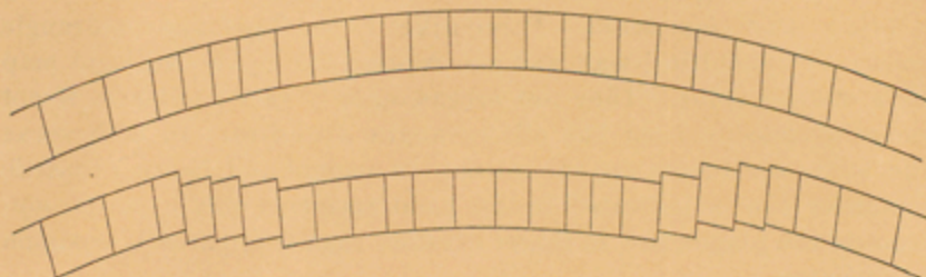
FIGURE 18.—An ideal arch broken into blocks by nearly vertical joint planes (upper figure) and the same arch as it would appear if the central part collapsed by displacement of the blocks along the joint planes, due to lack of support (lower figure).
