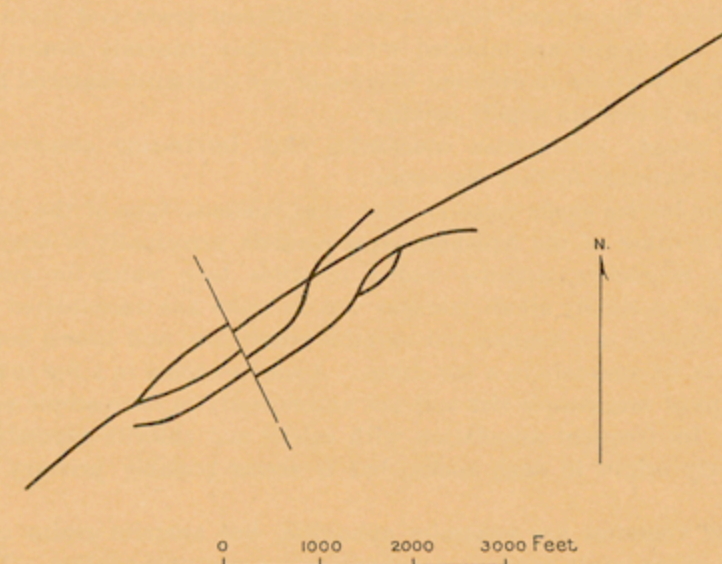
FIGURE 20.—Plan of dikes 2 miles northeast of North Rattlesnake Butte. By F. P. Gulliver. Shows branching and crossing of the dikes, and slight offset by faulting.
