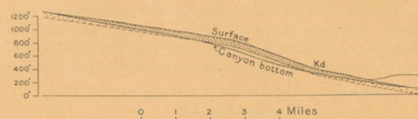
FIGURE 8.—Profiles of bottom of Crossbars Canyon and of surface of Dakota sandstone upland.
