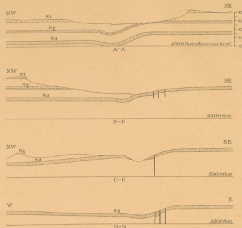
FIGURE 12.—Sections across Doyle Arroyo flexure.
