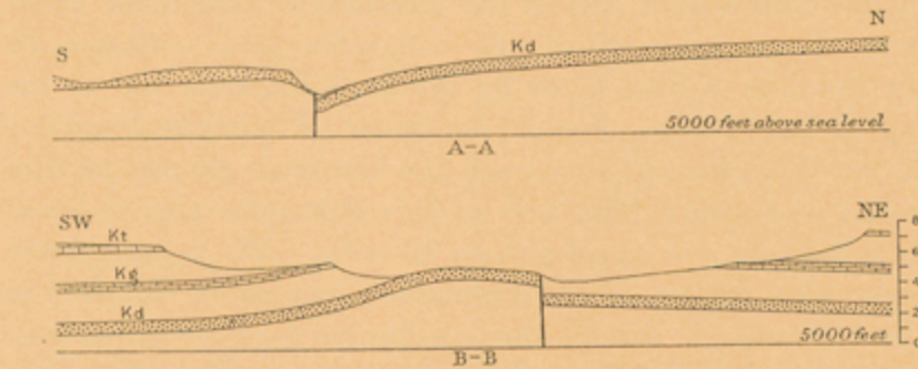
FIGURE 15.—Sections across Cross Canyon fault.
