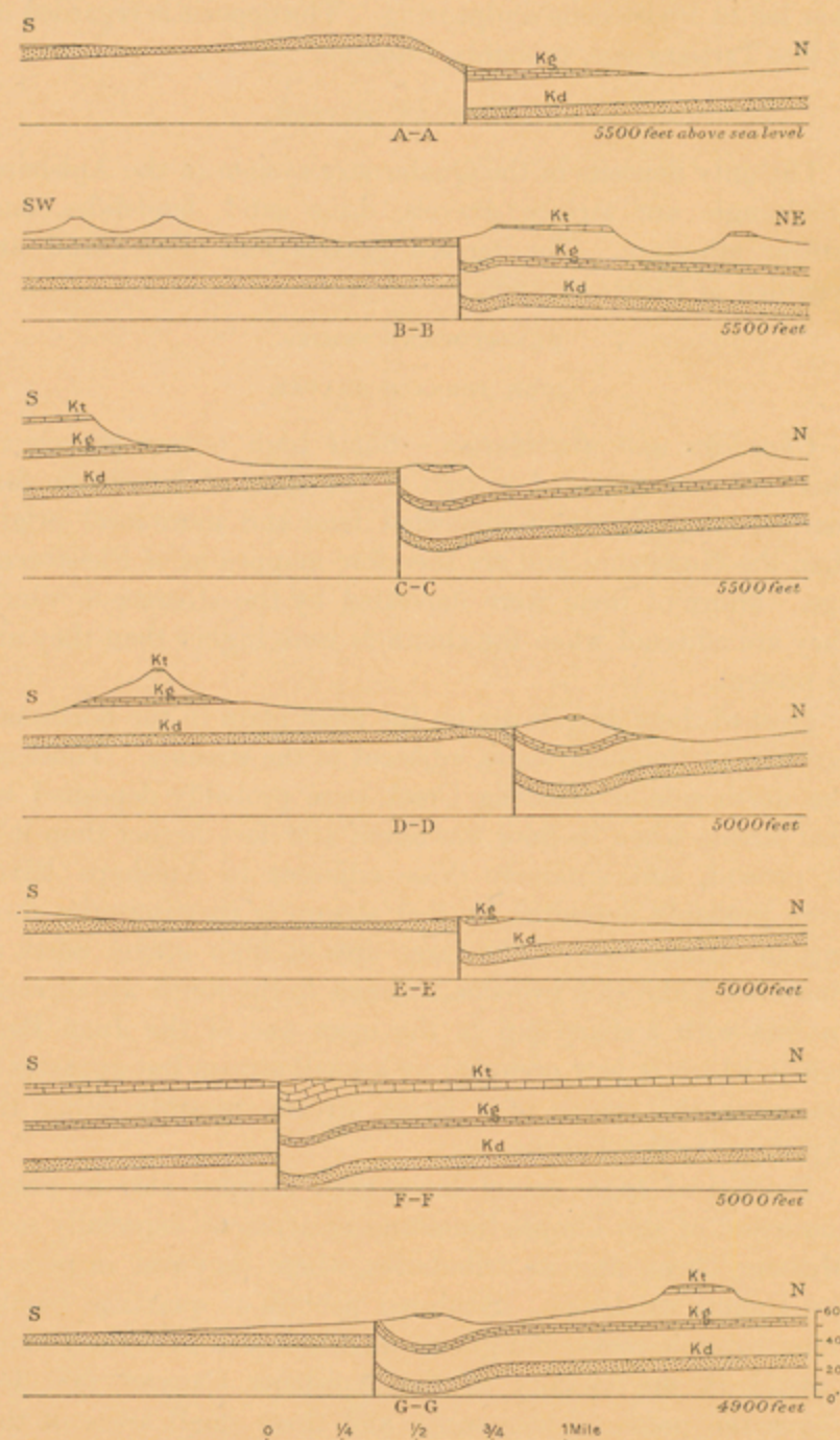
FIGURE 13.—Sections across Rocky Hill fault.
