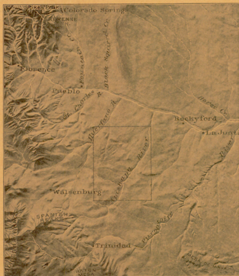
FIGURE 2.—Relief map of south-central Colorado.
