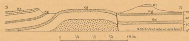
FIGURE 17.—Section across the Little Dome. Kd, Dakota sandstone; Kg, Greenhorn limestone; Kt, Timpas limestone. The strata beneath the Dakota are shown as having been intruded by a mass of igneous rock, which is believed to have domed up the overlying strata.
