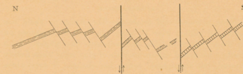
FIGURE 14.—Details of structure accompanying the Rocky Hill fault.
