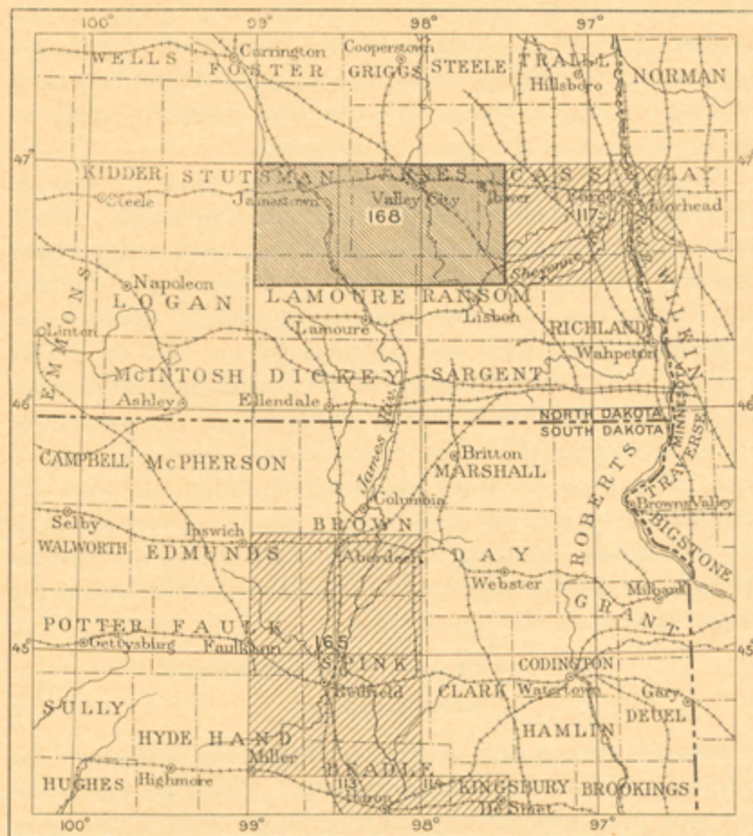
FIGURE 1.—Index map of the vicinity of the Jamestown-Tower district.
