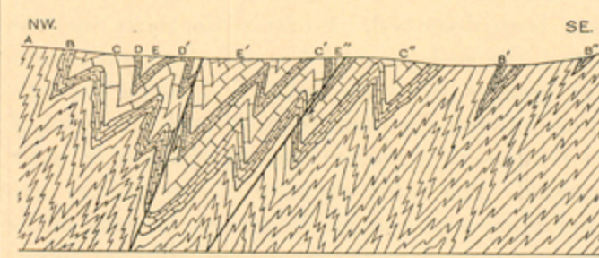
FIG. 1.—Ideal geologic section across the principal belt of Rockport limestone southwest of Rockland, Me. A, Sedimentary rocks underlying Rockport limestone; B, B', B'', magnesian limestone or dolomite; C, C', C'', "hard rock"; D, D', impure limestone; E, E', E'', "soft rock."
