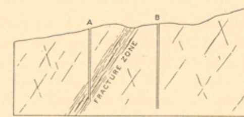
FIG. 2.—Diagrammatic section showing a well at A obtaining water from a fracture zone and a dry well at B.
