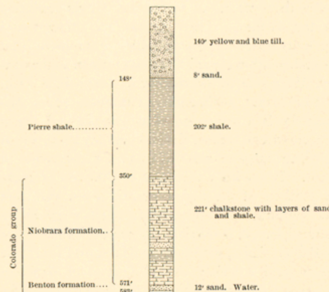
FIG. 6.—Section of well in SW 1/4 sec. 4, T. 107 N., R. 56 W.
