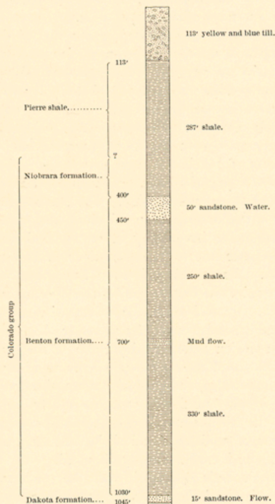
FIG. 2.—Section of Brooks well, NE 1/4 sec. 21, T. 112 N., R. 58 W.
