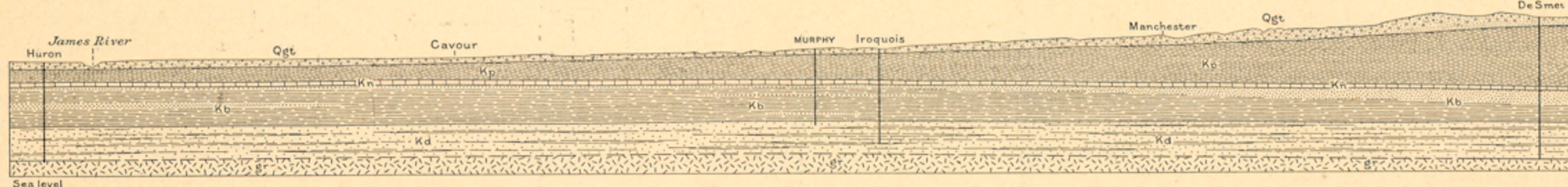
FIG. 1.—Sketch section from Huron to De Smet, showing the artesian wells extending to the Dakota water-bearing sandstone. Qgt, Glacial till; Kp, Pierre shale; Kc, Niobrara formation; Kd, Benton formation; Kd, Dakota formation; g, granite, including probably overlying Sioux quartzite in places. Horizontal scale: 1 inch = 3 miles. Vertical scale: 1 inch = 1500 feet.
