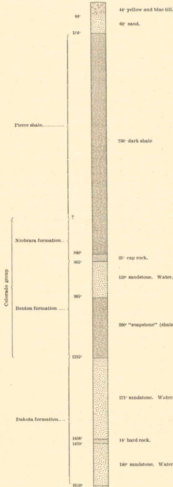
FIG. 5.—Section of well at De Smet.
