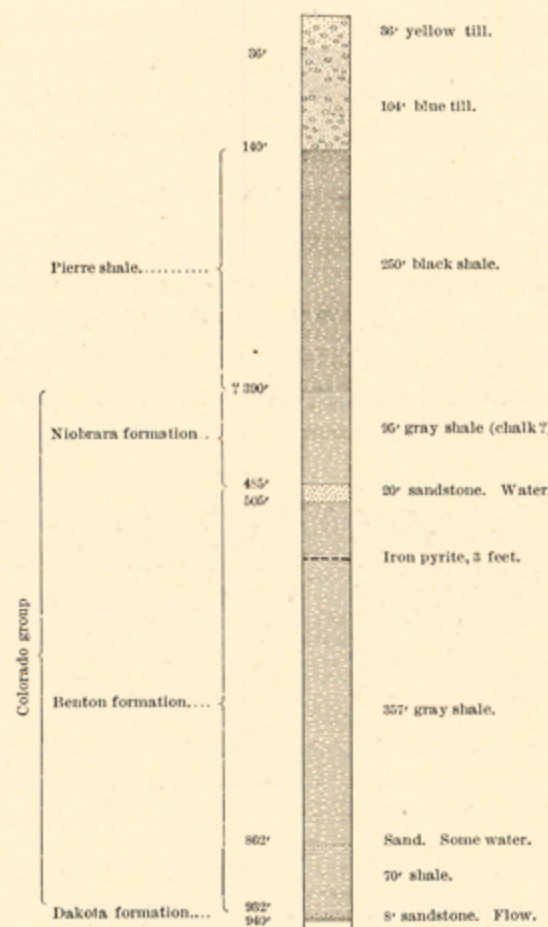
FIG. 4.—Section of Spear well, NE 1/4 sec. 19, T. 110 N., R. 57 W.
