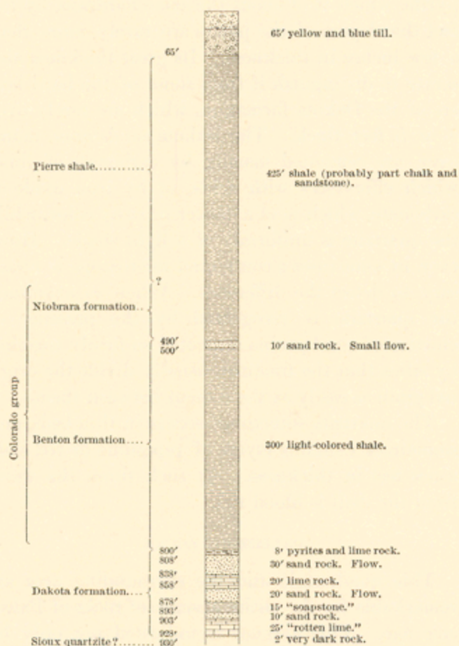
FIG. 2.—Section of Wolsey well. Sec. 24, T. 111, R. 64.
