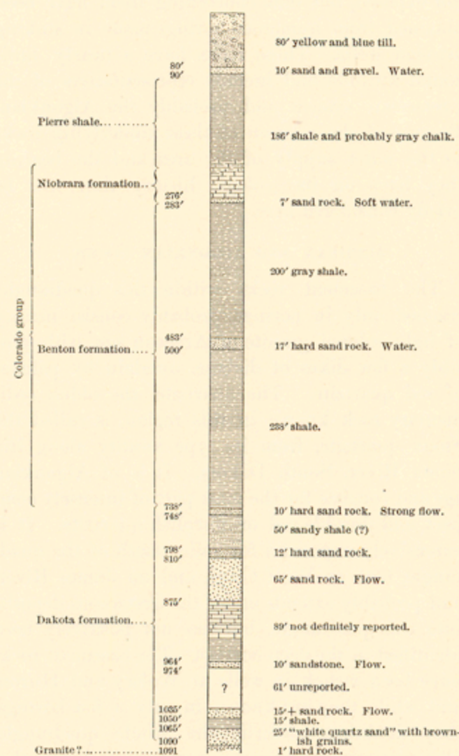
FIG. 3.—Section of Huron well No. 3. Sec. 1, T. 110, R. 61.
