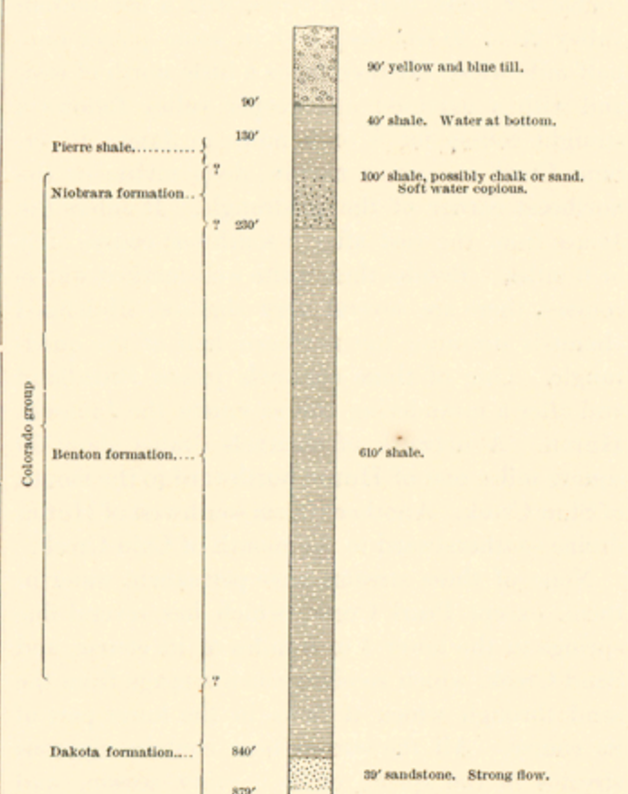
FIG. 4.—Section of well at Poor farm. Sec. 15, T. 110, R. 61.
