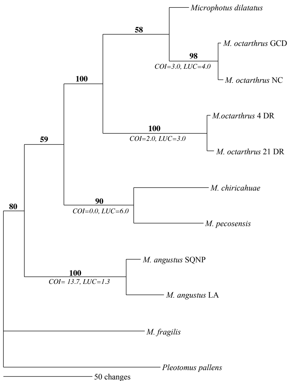
Fig. 8 Phylogeny of Microphotus species based on combined molecular data. The tree shown is 1 of 2 most parsimonious trees for combined mtCOI and luciferase data. CI= 0.8170, RI=0.6627. Bold numbers above branches indicate bootstrap values. Bootstrap values less than 50 indicate clades unresolved in strict consensus. Italicized numbers below branches indicate partitioned Bremer support (COI= mt cytochrome oxidase I, LUC = luciferase). Numbers following taxa indicate individuals. Letters following taxa indicate populations (GCD=New Mexico, Catron Co., Gila Nat'l. For.; NC= Arizona, Graham Co., Coronado Nat'l. Forest., Noon Creek; DR=Texas, Val Verde Co., Devils River State Natural Area; SQNP= California, Tulare Co., Sequoia Nat'l. Park, Potwisha; LA= California, Los Angeles Co., Los Angeles)
