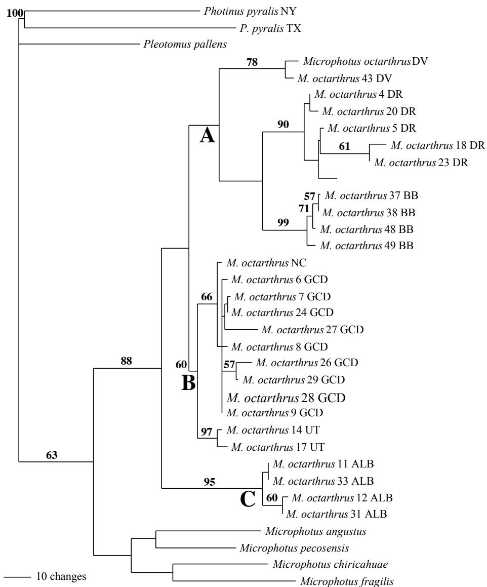
Fig. 9 Phylogeny of M. octarthrus populations based on mtCOI data. The tree shown is 1 of 15500 most parsimonious trees. CI=0.7024, RI=0.7536. Bootstrap values are given in bold above branches. Clades with bootstrap values lower than 50 are unresolved in strict consensus. Numbers following taxa indicate individuals. Letters following taxa indicate populations (NY=New York, Suffolk Co, Smithtown; TX=Texas, Fort Bend Co., Brazos Bend St. Park; DV=Texas, Jeff Davis Co., Davis Mts. St. Park; DR=Texas, Val Verde Co., Devil's River State Natural Area; BB= Texas, Presidio Co., Big Bend Nat'l. Park; NC=Arizona, Graham Co., Coranado Nat'l Forest, Noon Creek; GCD=New Mexico, Catron Co., Gila Nat'l. For.; UT=Utah, Washington Co., nr. Baker Dam Reservoir ; ALB=New Mexico, Bernalillo Co., nr. Albuquerque)
