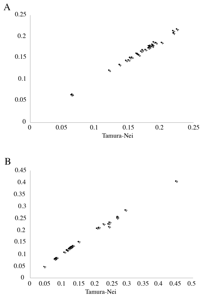
Fig.5 Tamura-Nei vs. Jukes-Cantor pairwise genetic distances. A=mtCOI, B=luciferase
