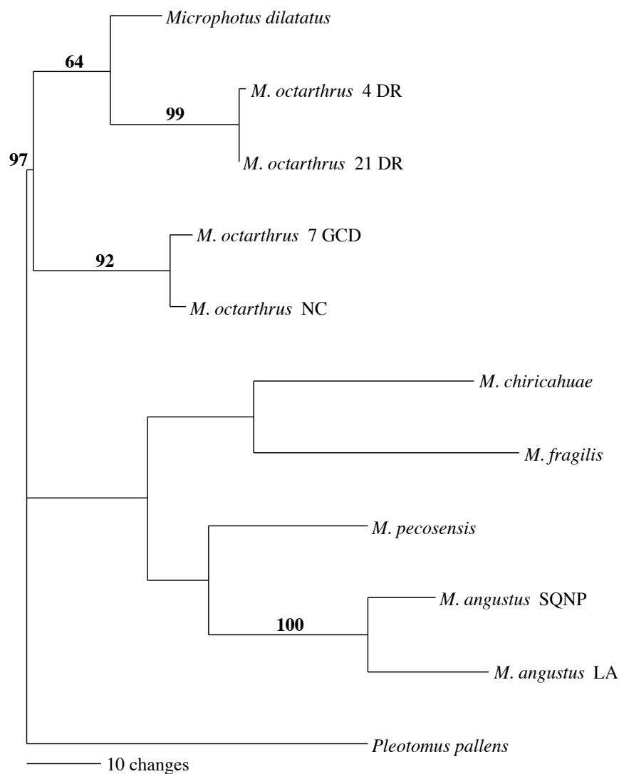
Fig. 6 Phylogeny of Microphotus species based on mtCOI data. The tree shown is 1 most parsimonious tree. CI=0.6611, RI=0.6164. Bold numbers above branches indicate bootstrap values. Numbers following taxa indicate individuals. Letters following taxa indicate populations (GCD= New Mexico, Catron Co., Gila Nat'l. For.; NC= Arizona, Graham Co., Coronado Nat'l. Forest., Noon Creek; DR=Texas, Val Verde Co., Devils River State Natural Area; SQNP= California, Tulare
