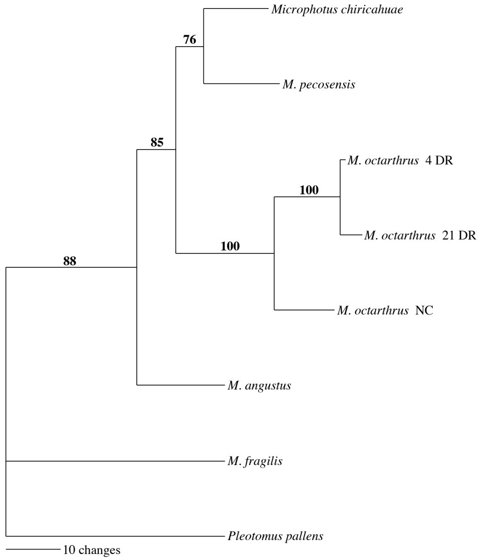
Fig. 7 Phylogeny of Microphotus species based on luciferase data. The single most parsimonious tree obtained is shown above. CI=0.9020, RI=0.7436. Bold numbers above branches indicate bootstrap values. Numbers following taxa indicate individuals. Letters following taxa indicate populations (NC= Arizona, Graham Co. Coronado Nat'l. Forest., Noon Creek;
