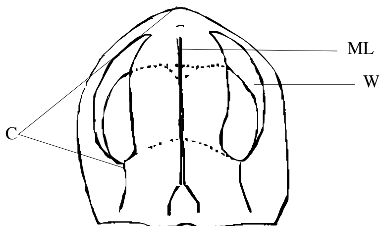
Fig 1. Pronotum of M. fragilis . C= convex area, ML=Median longitudinal line, W=windows (transparent spots)
