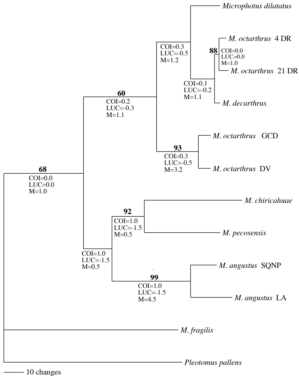
Fig.4 Phylogeny of Microphotus species based on combined morphological and molecular data. The tree shown is 1 of 2 most parsimonious trees for combined morphological and molecular data. CI=0.07861, RI=0.6556. Bold numbers above branches indicate bootstrap values. Bootstrap values less than 50 indicate clades unresolved in strict consensus. Numbers below branches indicate partitioned Bremer support (COI= mt cytochrome oxidase I, LUC = luciferase, M = morphology). Numbers following taxa indicate individuals. Letters following taxa indicate populations (GCD=New Mexico, Catron Co., Gila Nat'l. For.; NC= Arizona, Graham Co., Coronado Nat'l. Forest., Noon Creek; DR=Texas, Val Verde Co., Devils River State Natural Area; SQNP= California, Tilare Co., Sequoia Nat'l. Park, Potwisha; LA= California, Los Angeles Co., Los Angeles)
