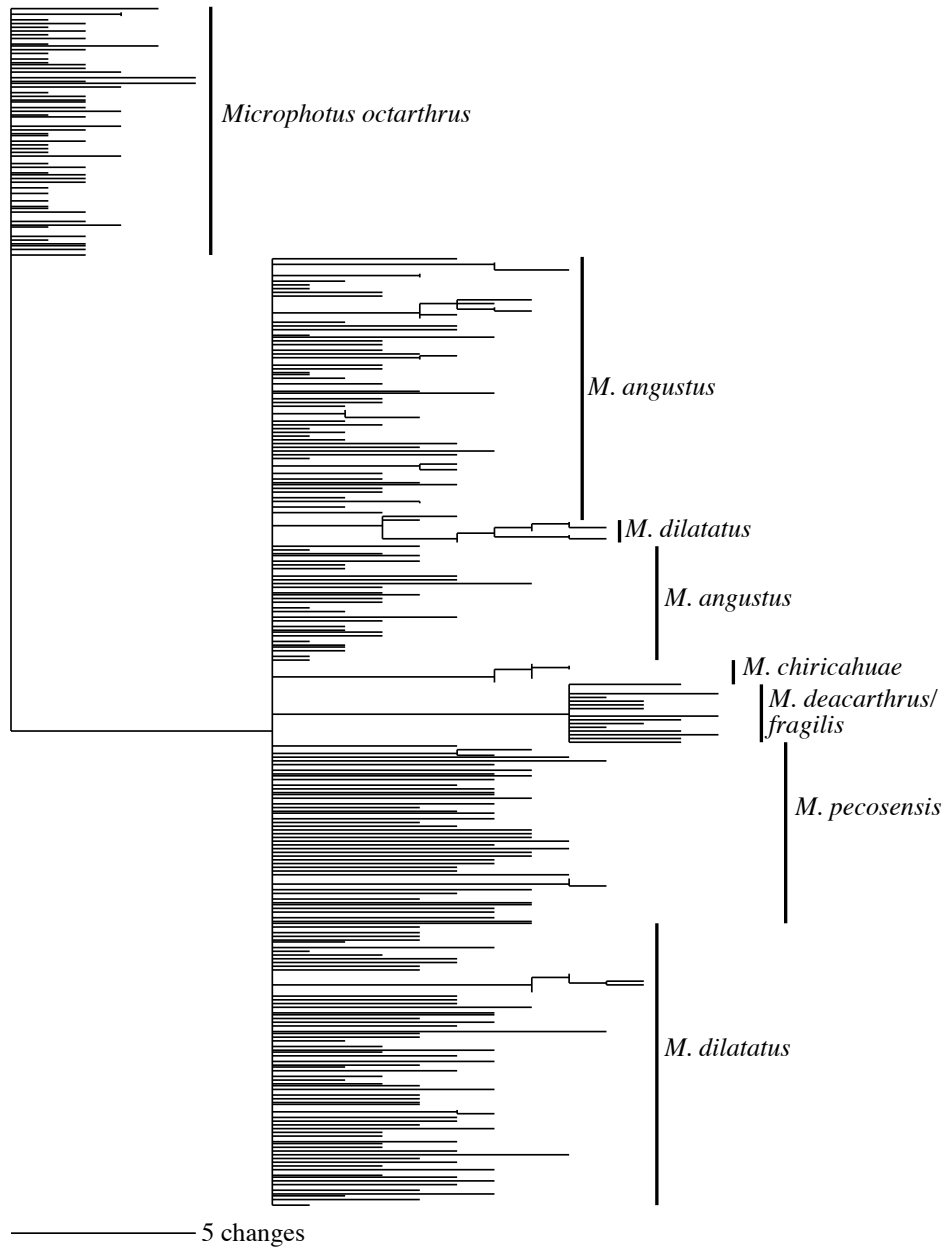
Fig.3 Phylogeny of Microphotus individuals based on morphological data. The tree shown is a strict consensus of 5000 trees (CI=0.445, RI=0.6626). Branches represent individuals.
