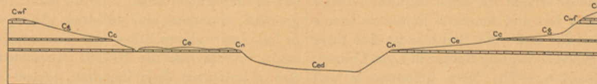
Fig. 1.—Northwest-southeast section across Cottonwood River 3 miles southwest of Elmdale. Shows the terraces and scarps produced by the limestone beds and the gentler slopes composed of shales. Cmf, Matfield shale; Cw, Wreford limestone; Cg, Garrison formation; Cc, Cottonwood limestone; Ce, Eskridge shale; Cn, Nevada limestone; Cd, Elmdale formation. Horizontal scale: 1 inch = 1 mile. Vertical scale: 1 inch = approximately 500 feet.
